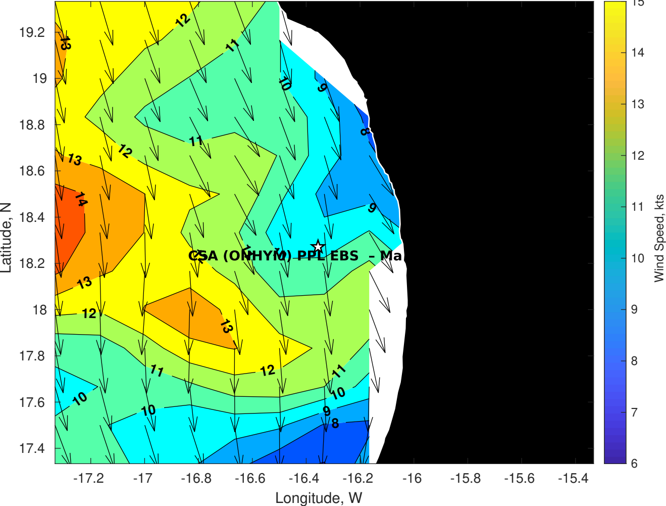
Winds (kts) for CSA (ONHYM) PPL EBS - Mauritania at 04-May-2025 09:00:00
