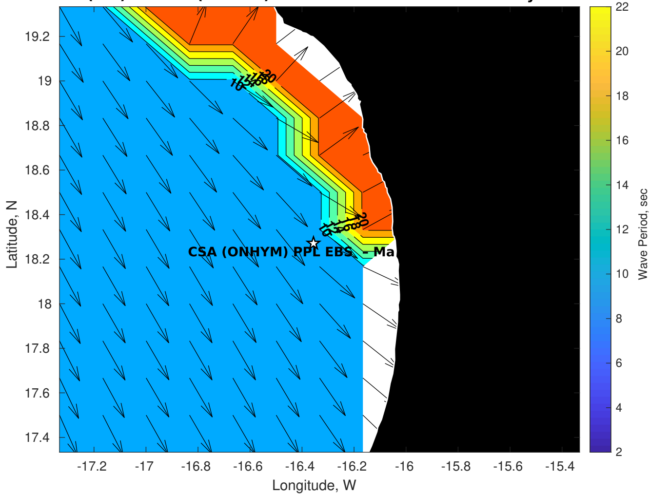
Wave Period (sec) for CSA (ONHYM) PPL EBS - Mauritania at 04-May-2025 09:00:00
