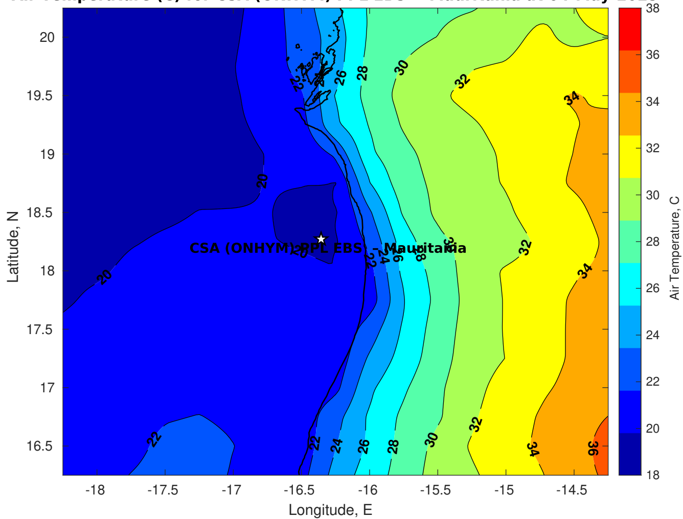
Air Temperature (C) for CSA (ONHYM) PPL EBS - Mauritania at 04-May-2025
