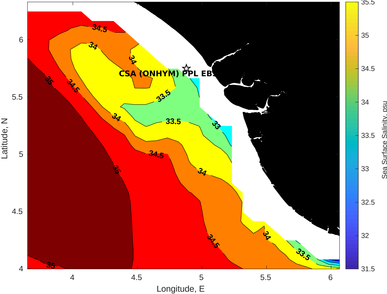
Surface Salinity for CSA (ONHYM) PPL EBS - Nigeria at 03-May-2025 00:00:00
