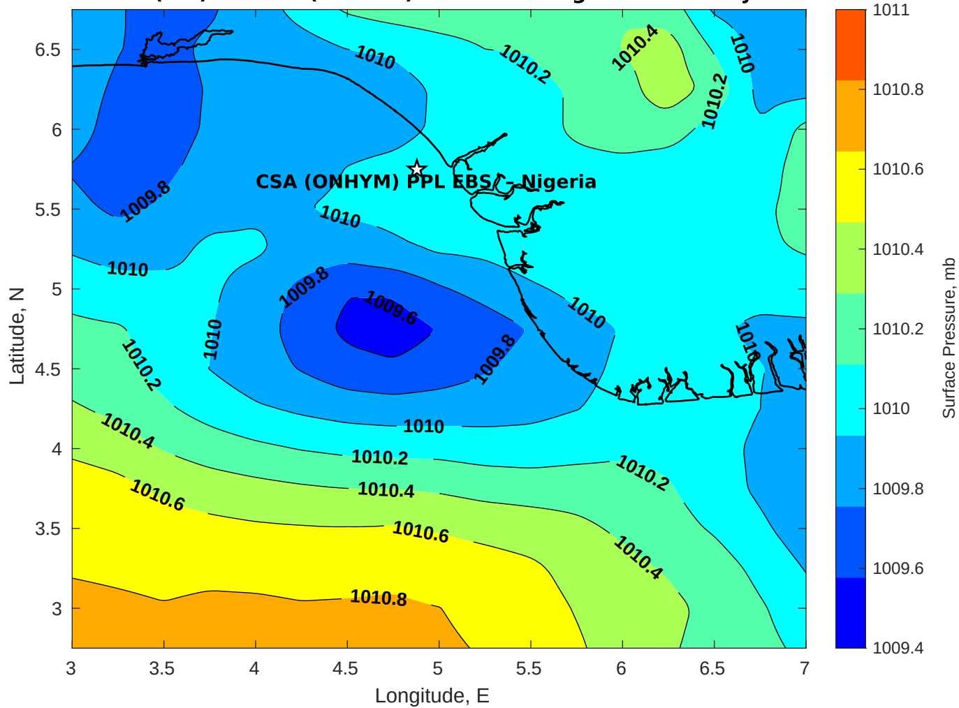
Surface Pressure (mb) for CSA (ONHYM) PPL EBS - Nigeria at 05-May-2025 00:00:00
