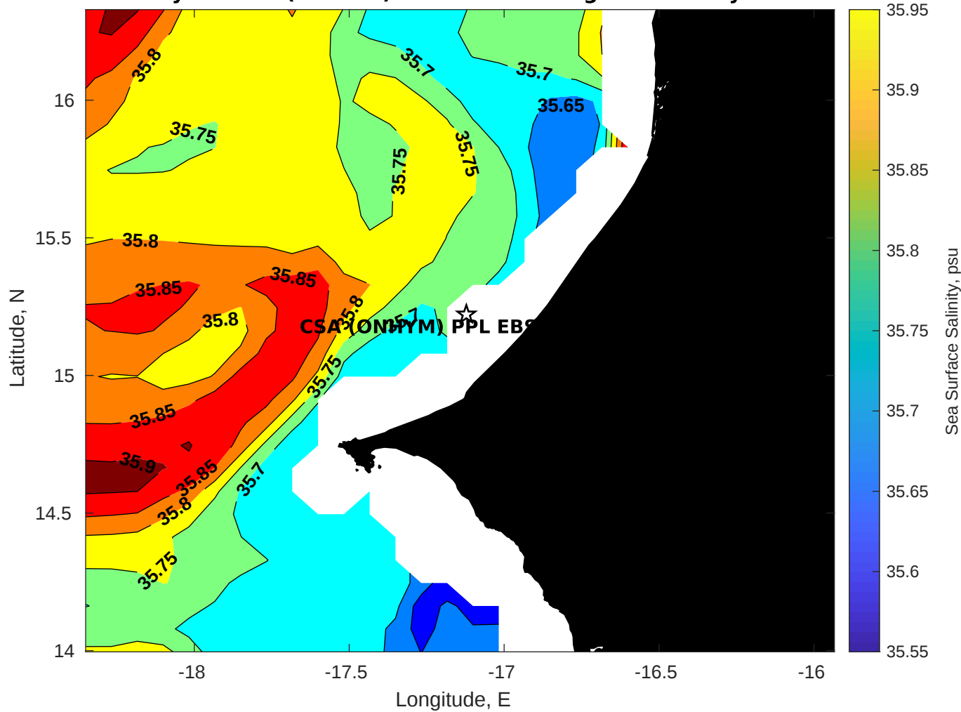
Surface Salinity for CSA (ONHYM) PPL EBS - Senegal at 03-May-2025 00:00:00
