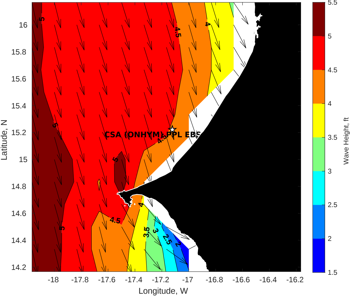
Wave Height (ft) for CSA (ONHYM) PPL EBS - Senegal at 04-May-2025 09:00:00
