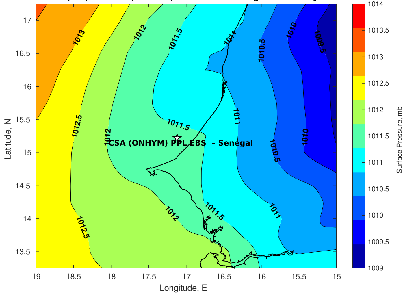
Surface Pressure (mb) for CSA (ONHYM) PPL EBS - Senegal at 06-May-2025 00:00:00
