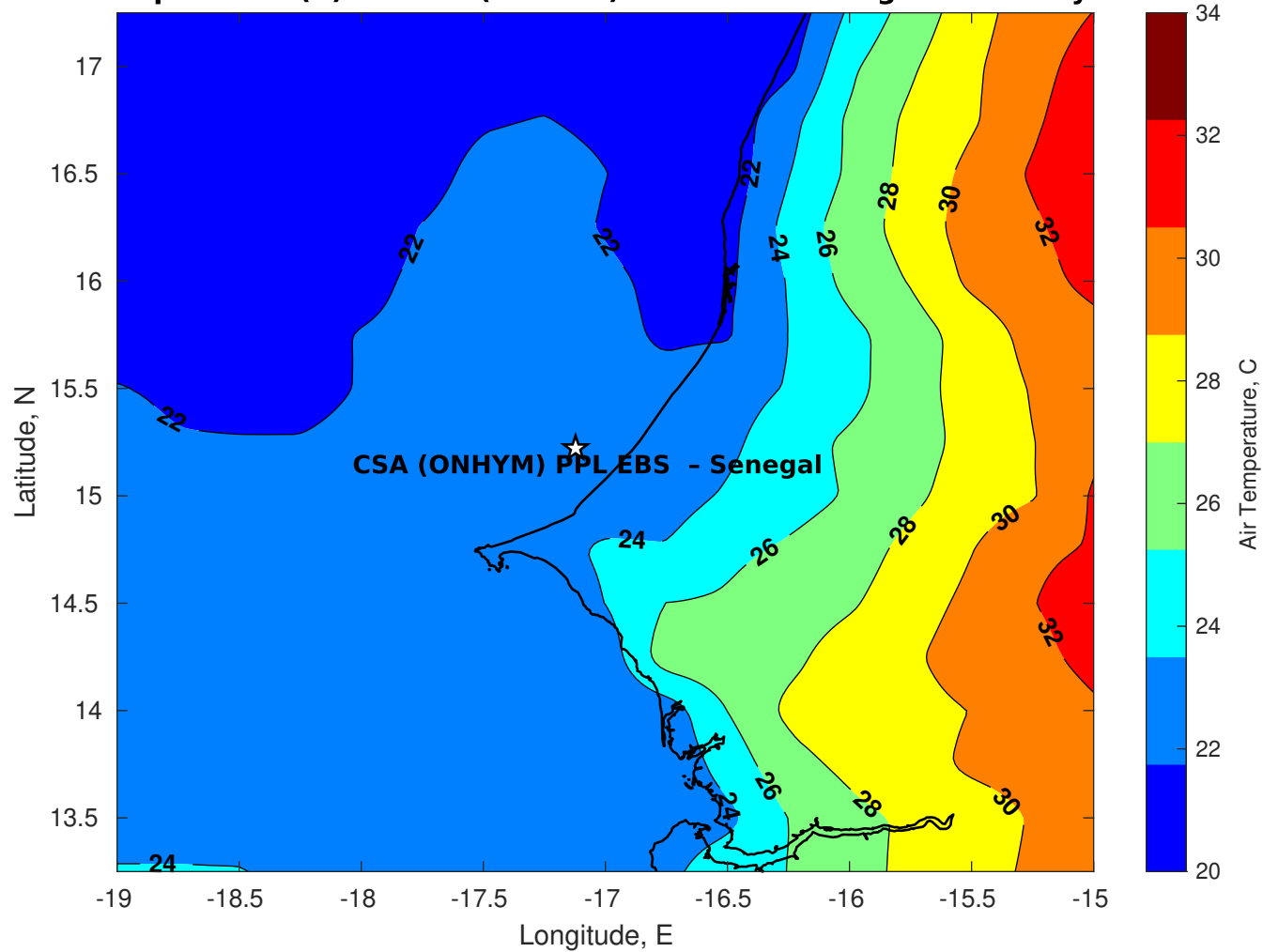
Air Temperature (C) for CSA (ONHYM) PPL EBS - Senegal at 04-May-2025
