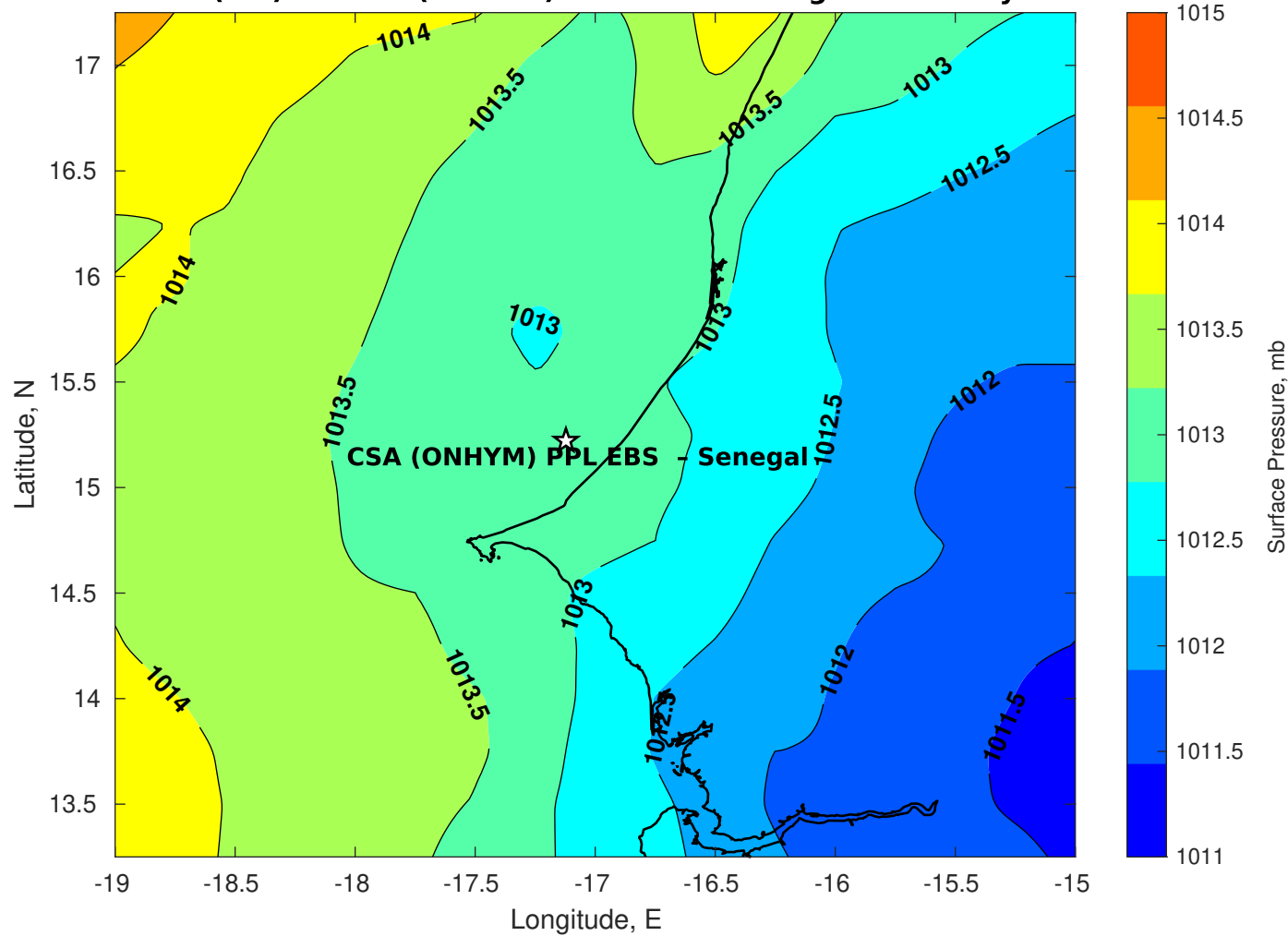
Surface Pressure (mb) for CSA (ONHYM) PPL EBS - Senegal at 04-May-2025 00:00:00
