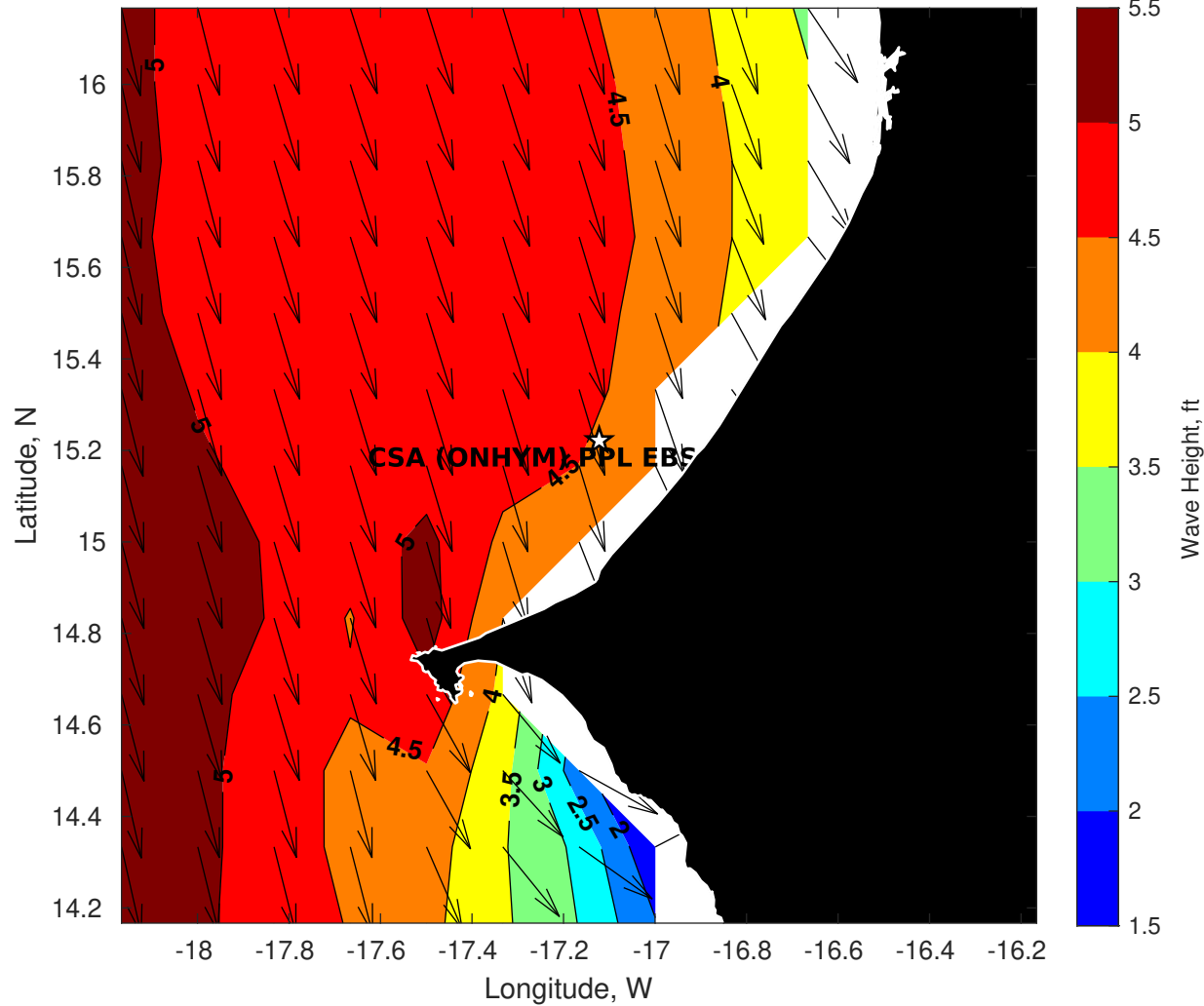
Wave Height (ft) for CSA (ONHYM) PPL EBS - Senegal at 04-May-2025 09:00:00
