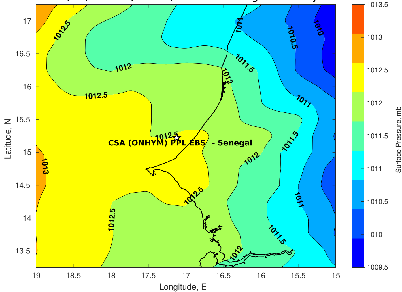
Surface Pressure (mb) for CSA (ONHYM) PPL EBS - Senegal at 05-May-2025 00:00:00
