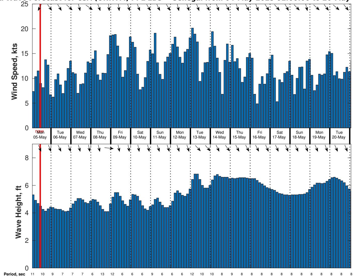
Wind & Wave Forecast for CSA (ONHYM) PPL EBS - Senegal from 04-May-2025 01:00:00 to 20-May-2025 01:00:00
