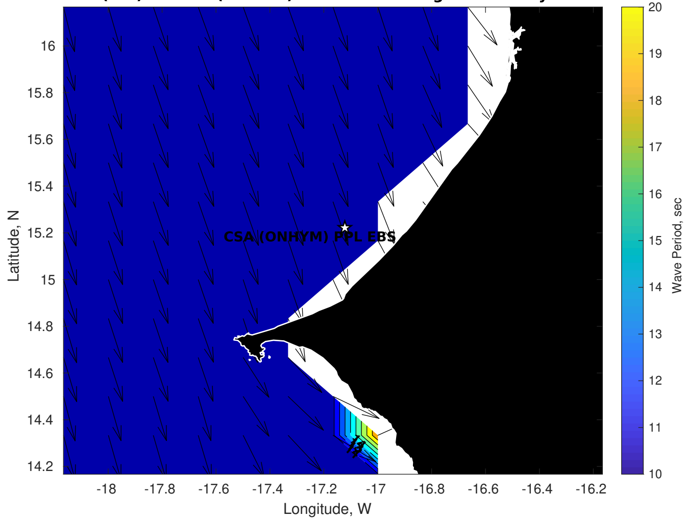
Wave Period (sec) for CSA (ONHYM) PPL EBS - Senegal at 04-May-2025 09:00:00
