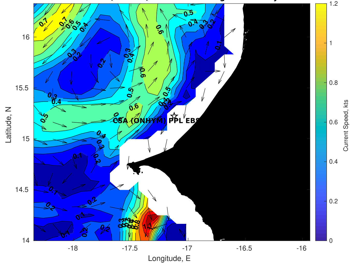
Surface Currents for CSA (ONHYM) PPL EBS - Senegal at 03-May-2025 00:00:00
