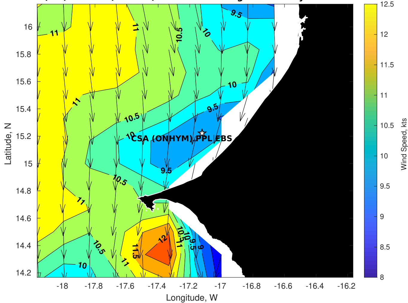
Winds (kts) for CSA (ONHYM) PPL EBS - Senegal at 04-May-2025 09:00:00
