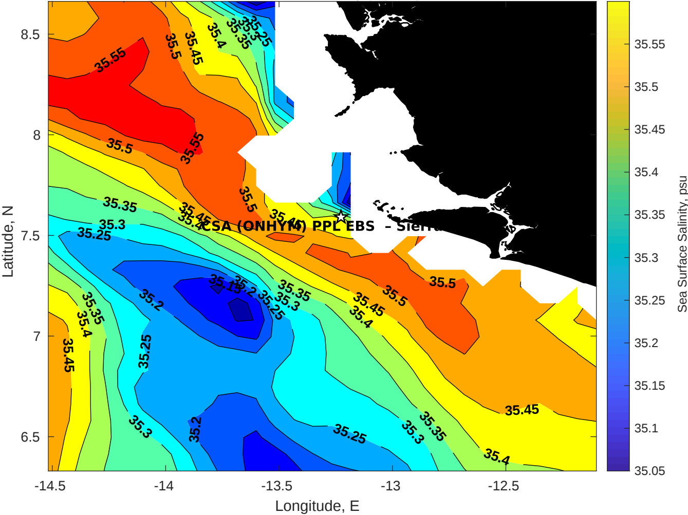
Surface Salinity for CSA (ONHYM) PPL EBS - Sierra Leone at 03-May-2025 00:00:00
