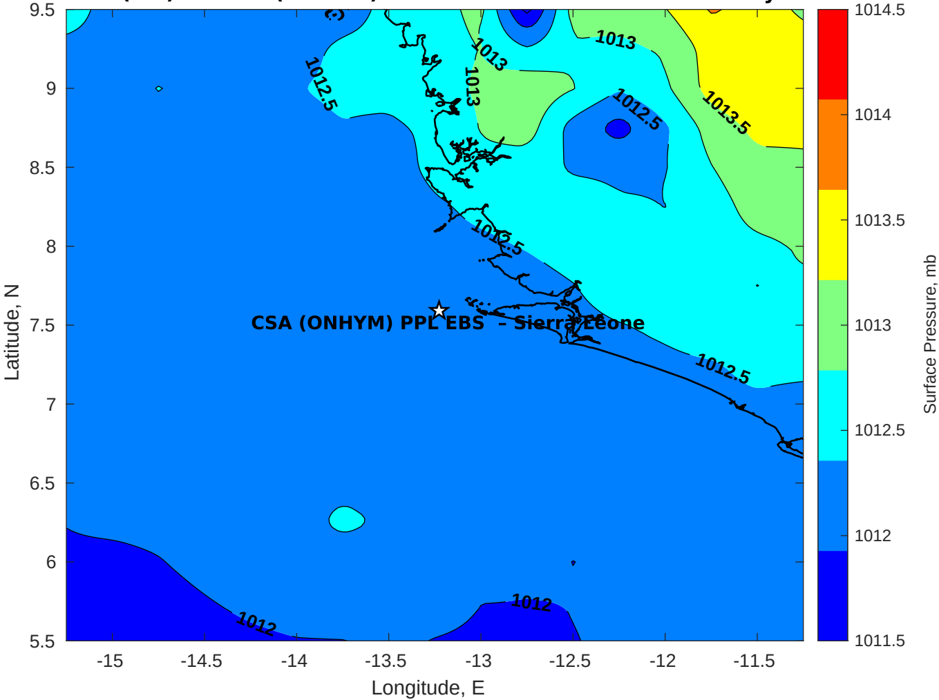
Surface Pressure (mb) for CSA (ONHYM) PPL EBS - Sierra Leone at 06-May-2025 00:00:00
