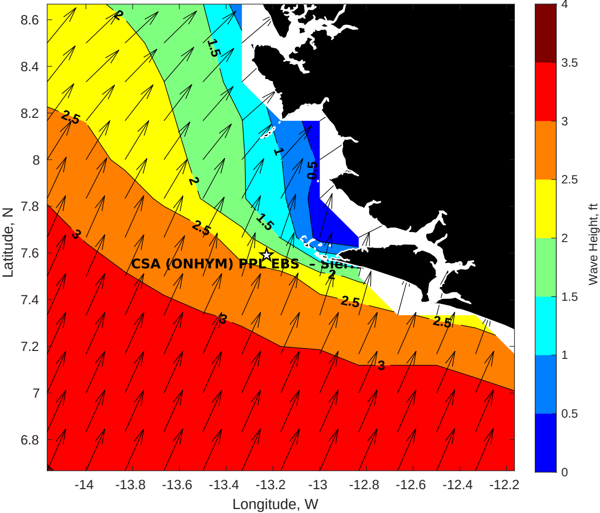
Wave Height (ft) for CSA (ONHYM) PPL EBS - Sierra Leone at 04-May-2025 09:00:00
