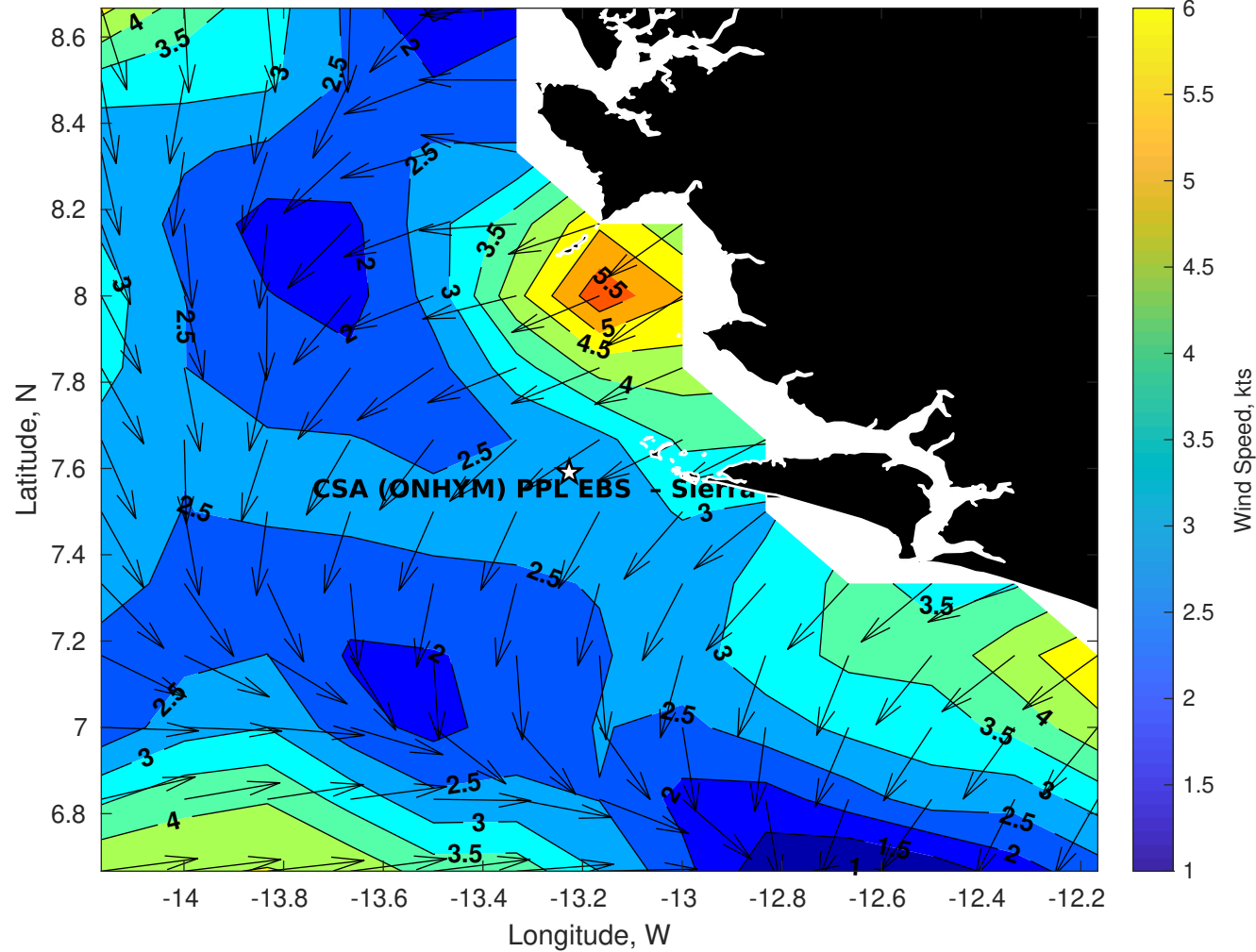
Winds (kts) for CSA (ONHYM) PPL EBS - Sierra Leone at 04-May-2025 09:00:00
