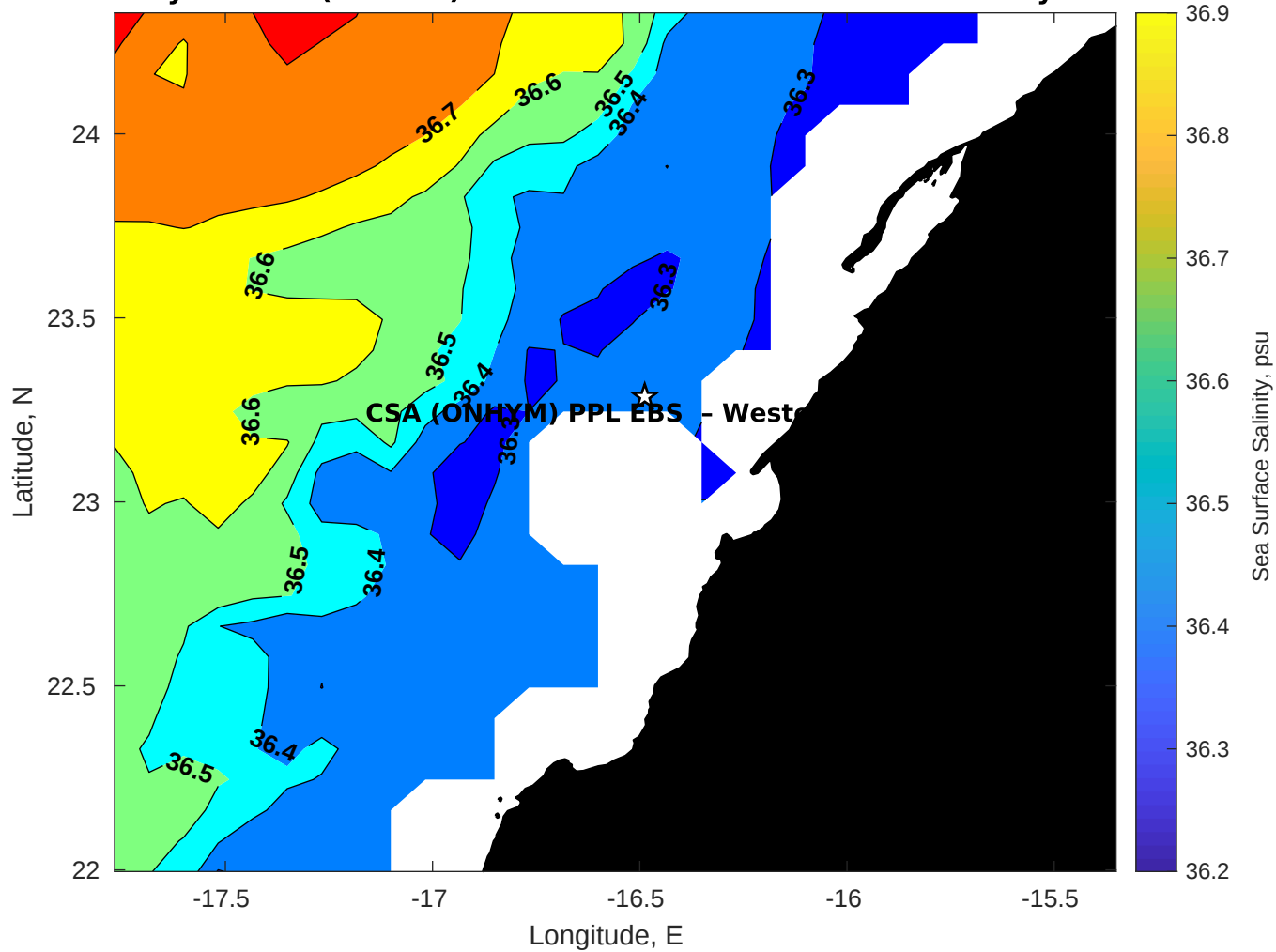
Surface Salinity for CSA (ONHYM) PPL EBS - Western Sahara at 03-May-2025 00:00:00
