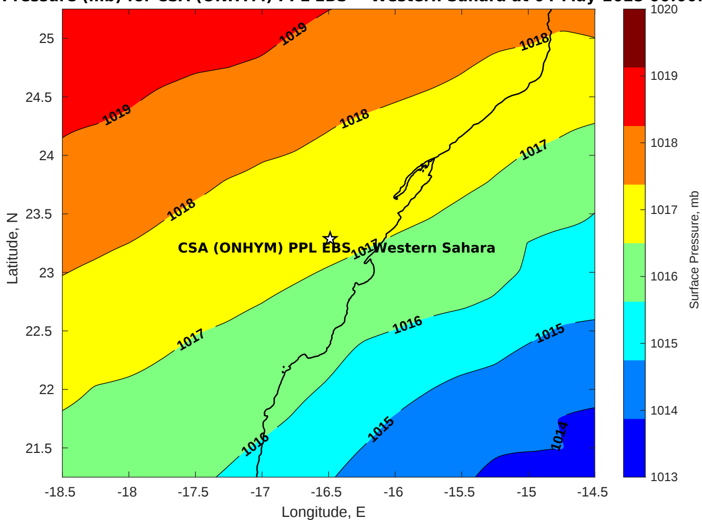
Surface Pressure (mb) for CSA (ONHYM) PPL EBS - Western Sahara at 04-May-2025 00:00:00
