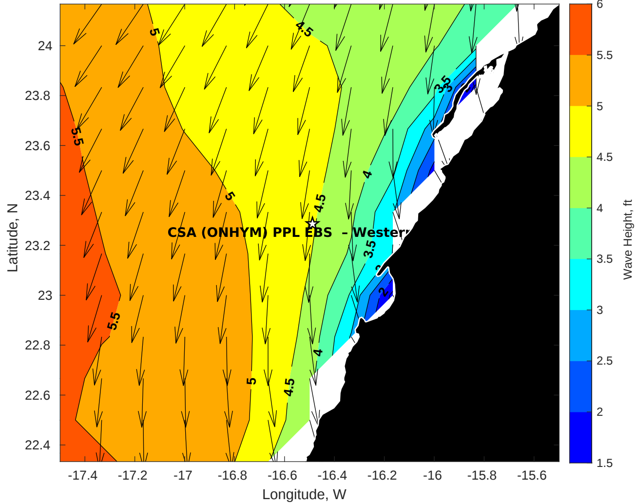
Wave Height (ft) for CSA (ONHYM) PPL EBS - Western Sahara at 04-May-2025 09:00:00
