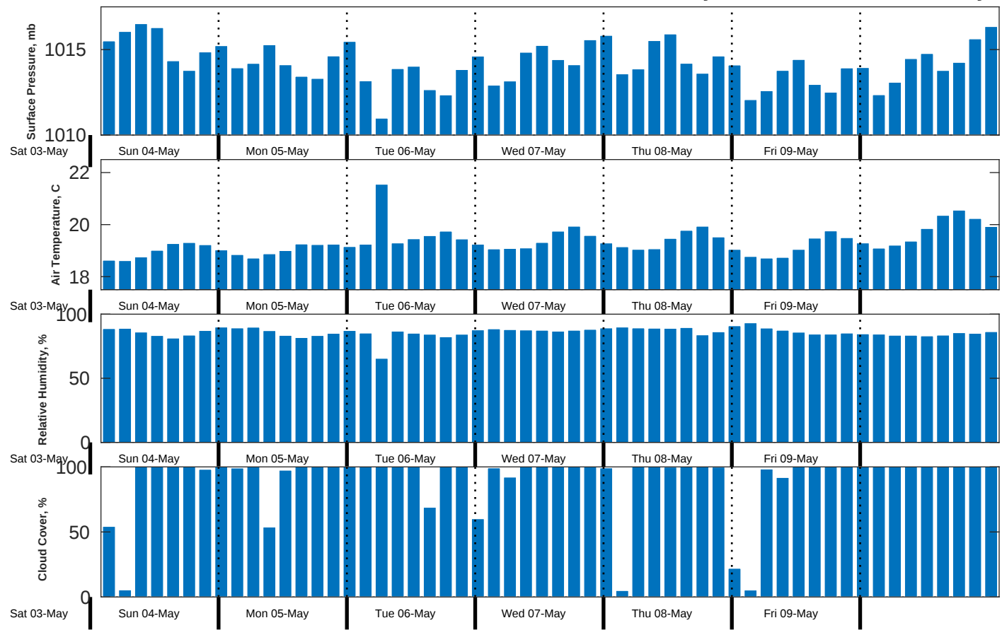
Met Forecast for CSA (ONHYM) PPL EBS - Western Sahara from 04-May-2025 00:00:00 to 11-May-2025 00:00:00
