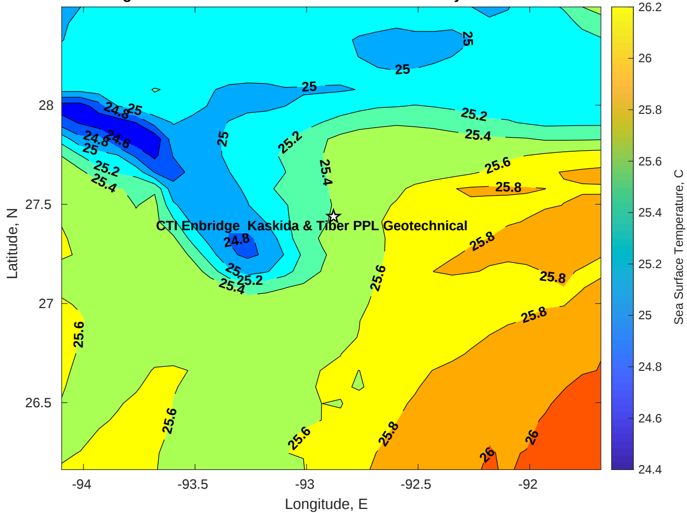
SST for CTI Enbridge Kaskida & Tiber PPL Geotechnical at 03-May-2025 00:00:00
