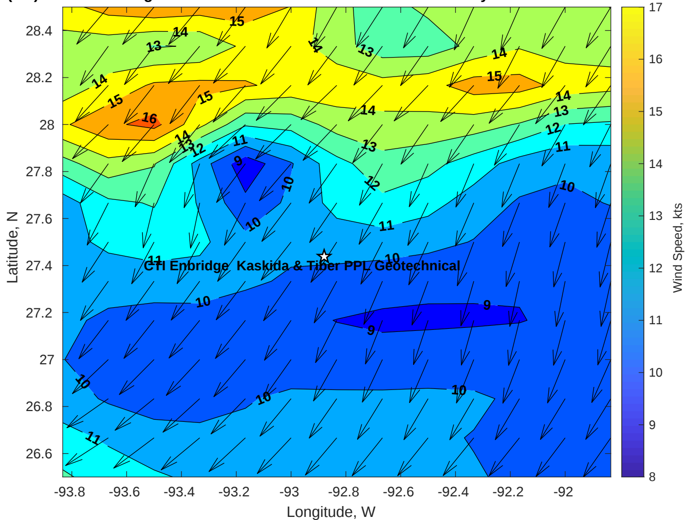
Winds (kts) for CTI Enbridge Kaskida & Tiber PPL Geotechnical at 04-May-2025 09:00:00
