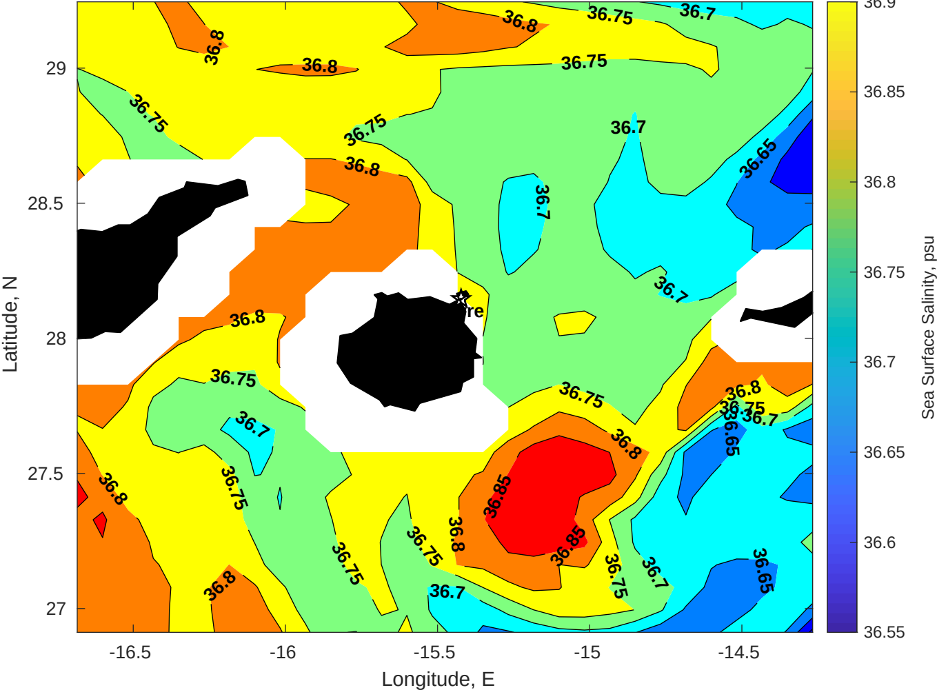
Surface Salinity for Gyre at 03-May-2025 00:00:00
