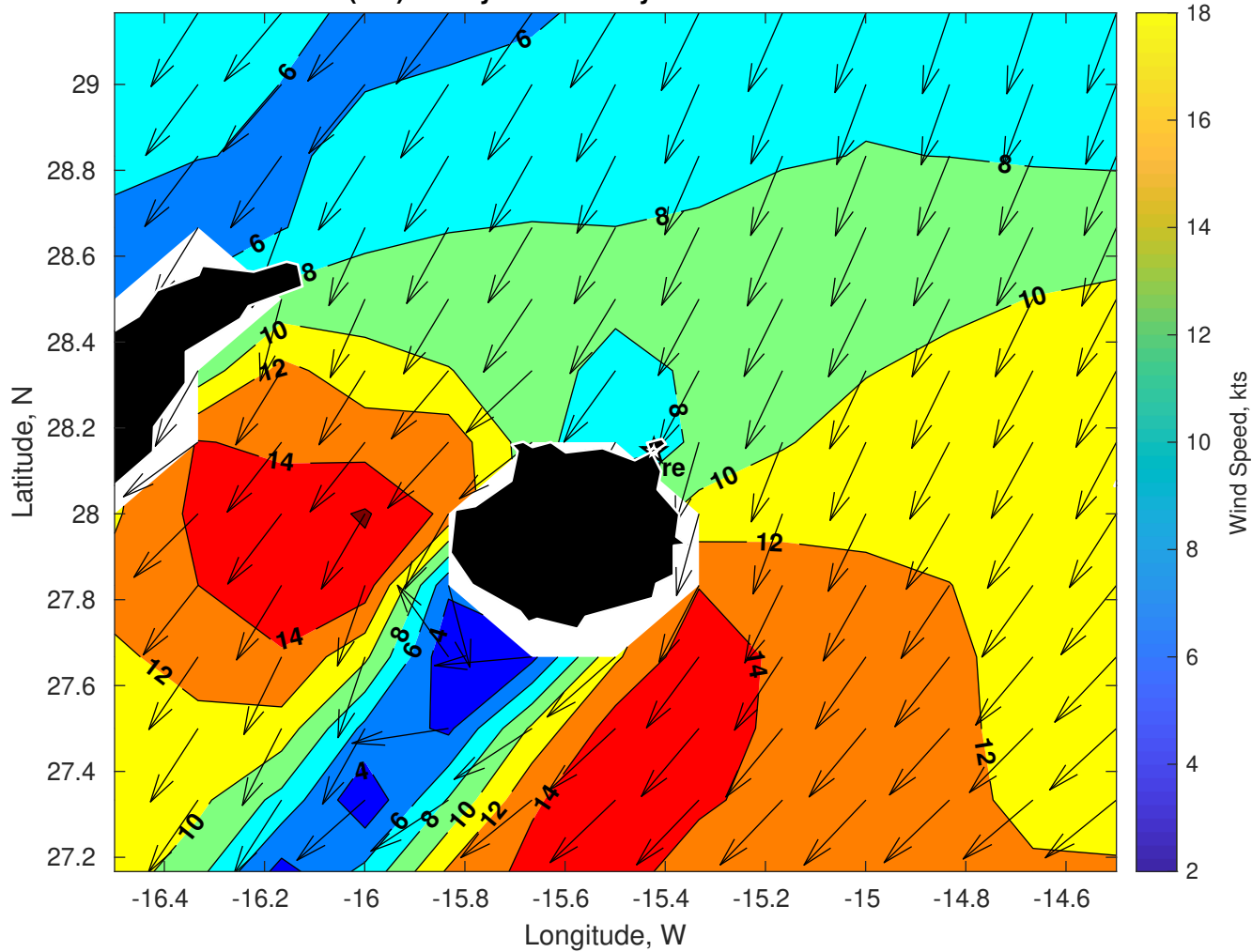
Winds (kts) for Gyre at 04-May-2025 09:00:00
