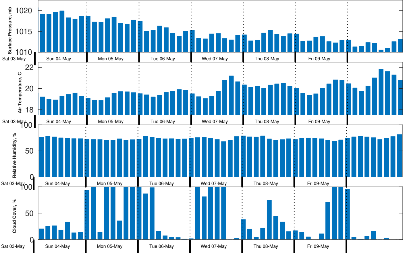
Met Forecast for Gyre from 03-May-2025 23:00:00 to 10-May-2025 23:00:00
