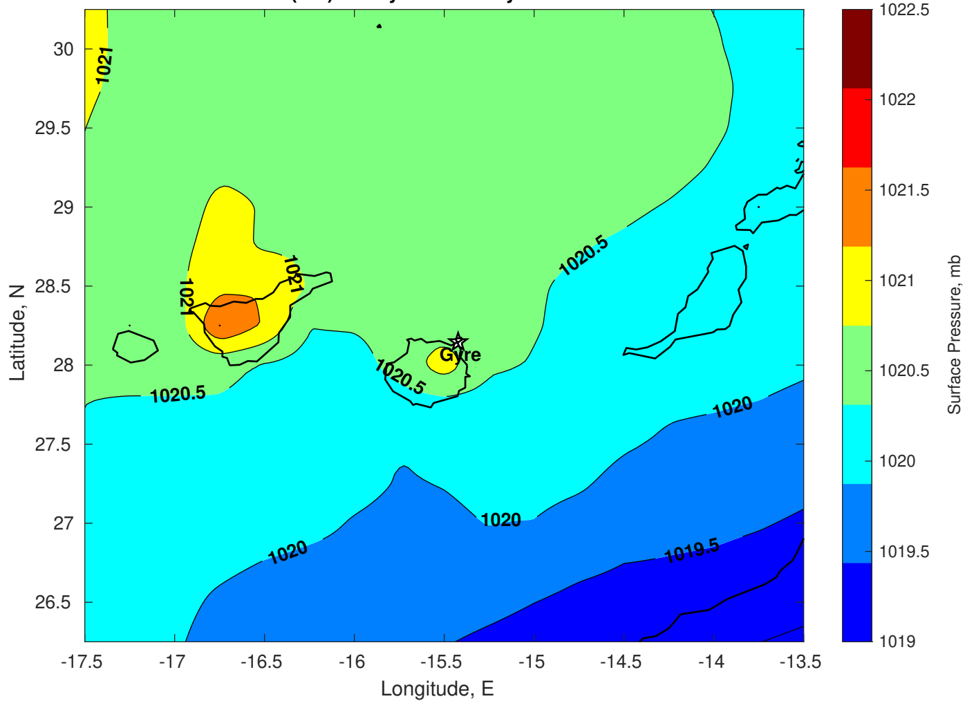
Surface Pressure (mb) for Gyre at 04-May-2025 00:00:00
