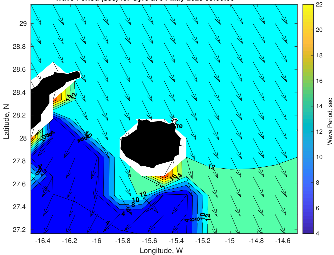
Wave Period (sec) for Gyre at 04-May-2025 09:00:00
