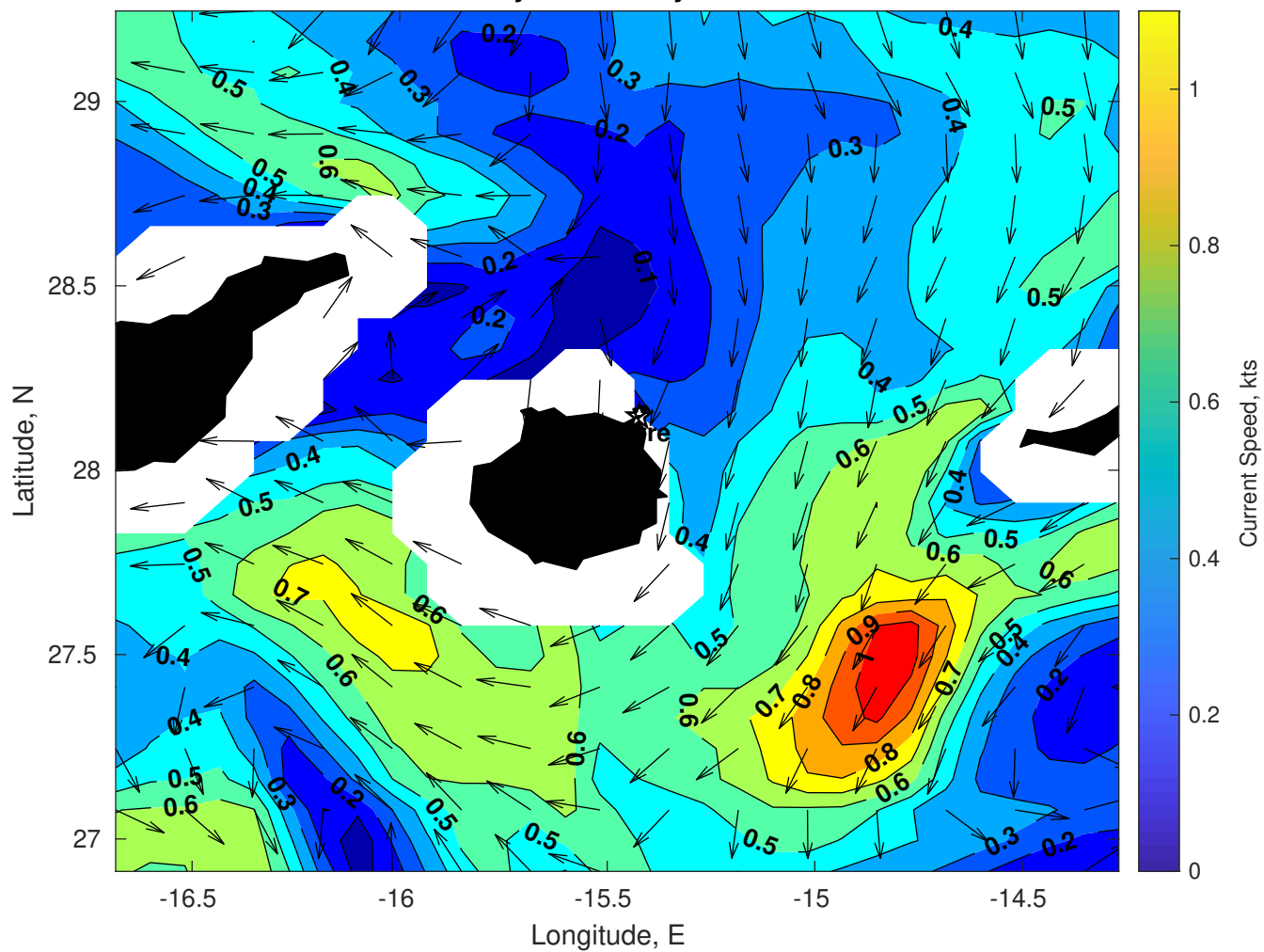
Surface Currents for Gyre at 03-May-2025 00:00:00
