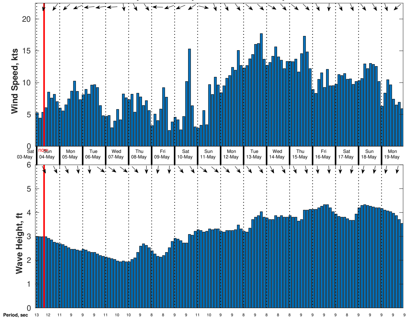
Wind & Wave Forecast for Gyre from 03-May-2025 23:00:00 to 19-May-2025 23:00:00
