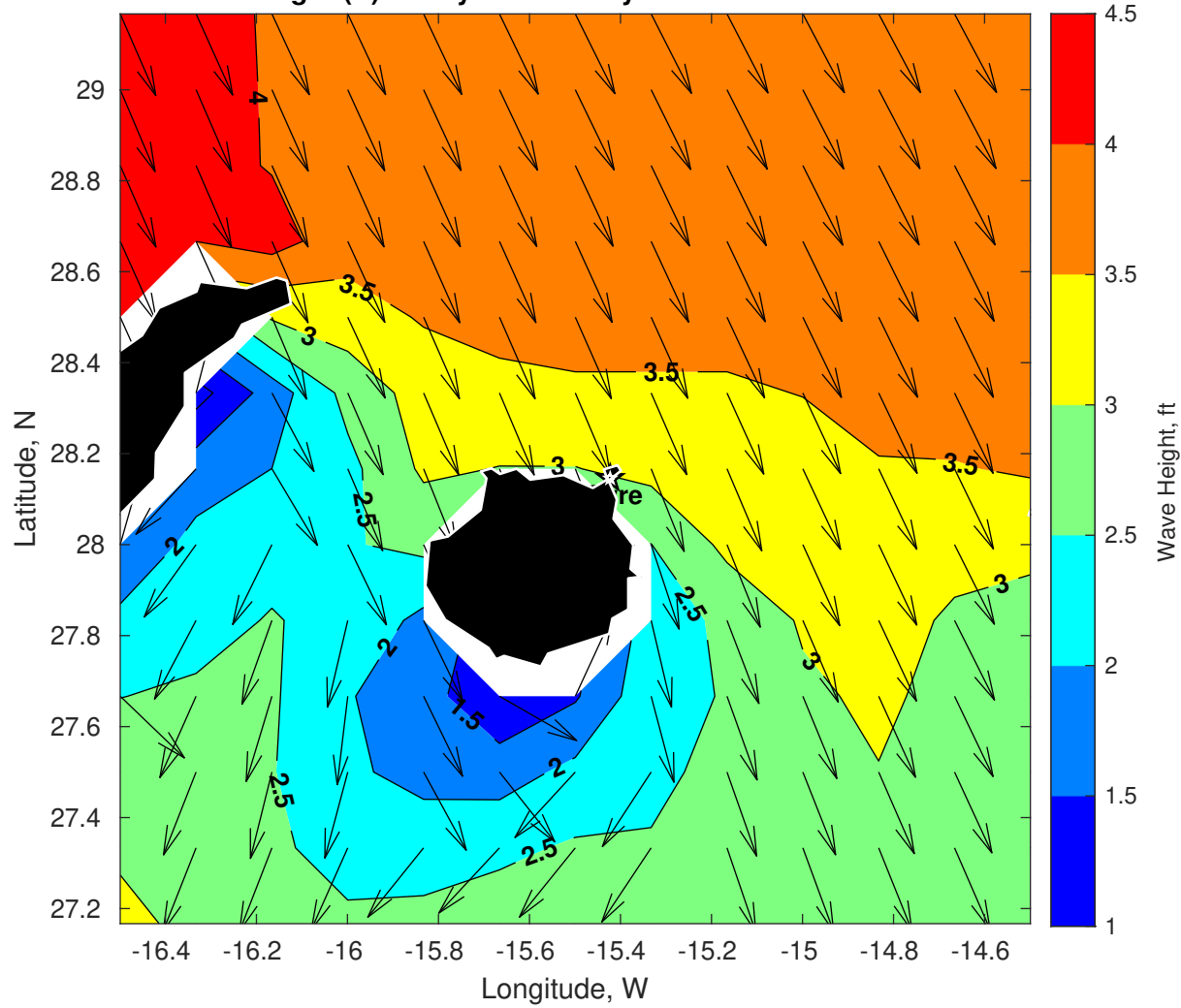
Wave Height (ft) for Gyre at 04-May-2025 09:00:00
