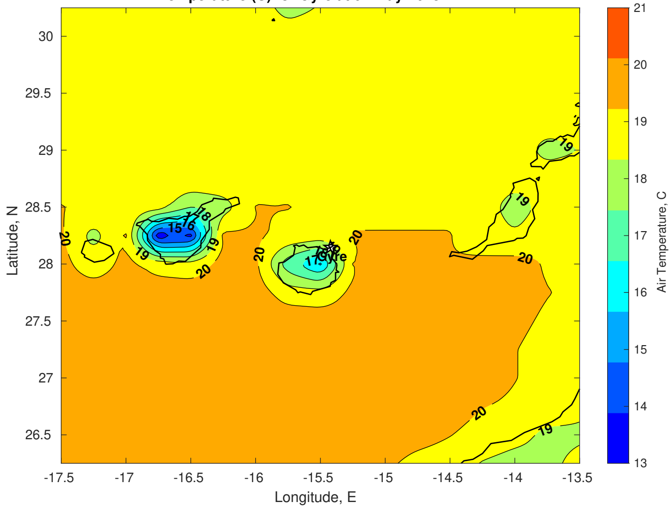
Air Temperature (C) for Gyre at 04-May-2025
