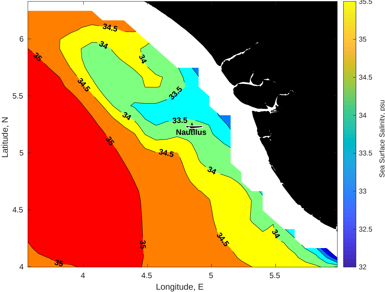
Surface Salinity for Nautilus at 03-May-2025 00:00:00
