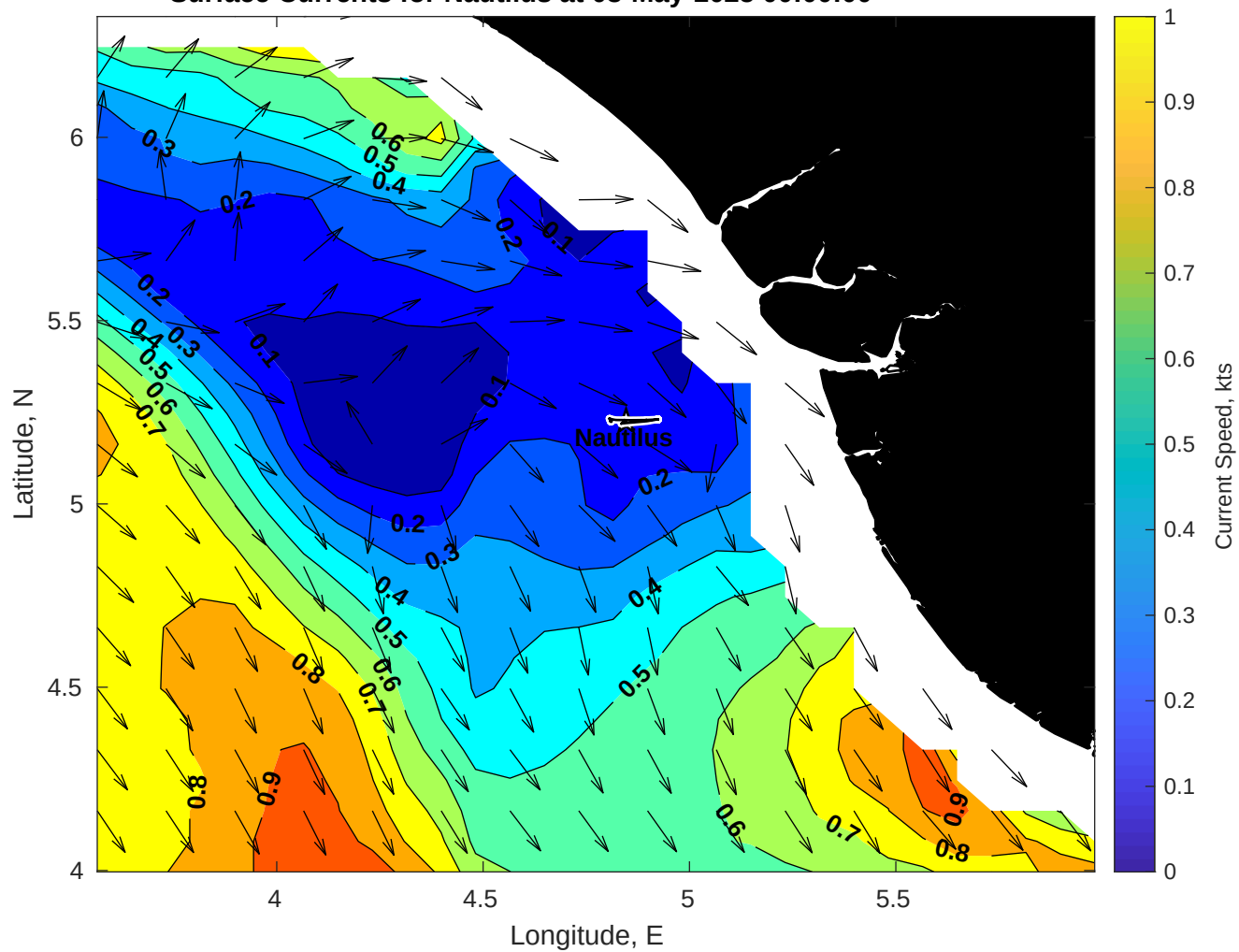
Surface Currents for Nautilus at 03-May-2025 00:00:00
