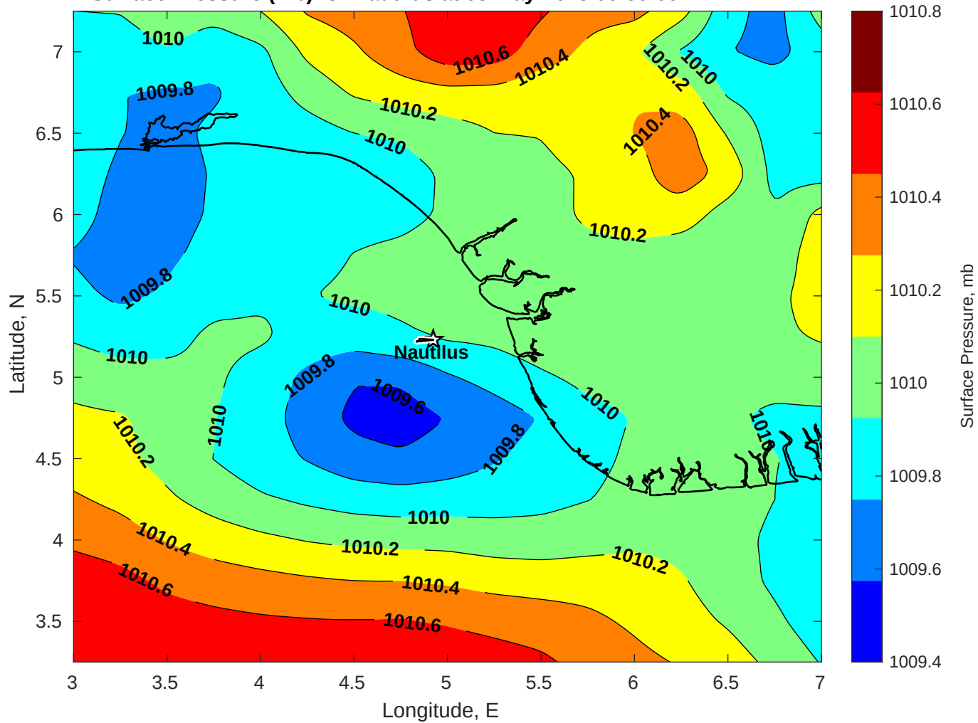
Surface Pressure (mb) for Nautilus at 05-May-2025 00:00:00
