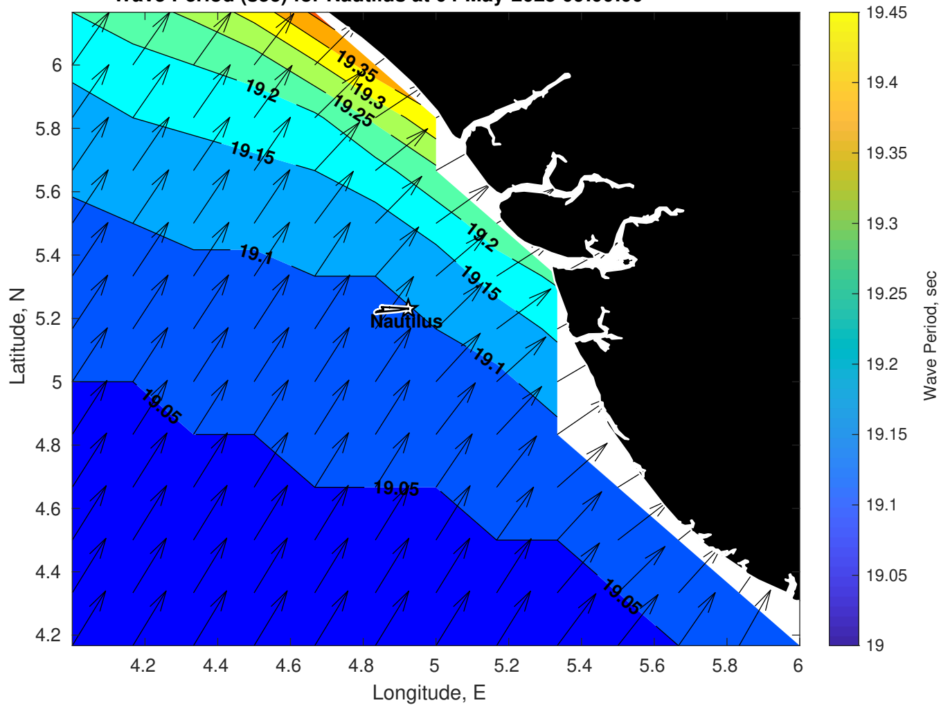
Wave Period (sec) for Nautilus at 04-May-2025 09:00:00
