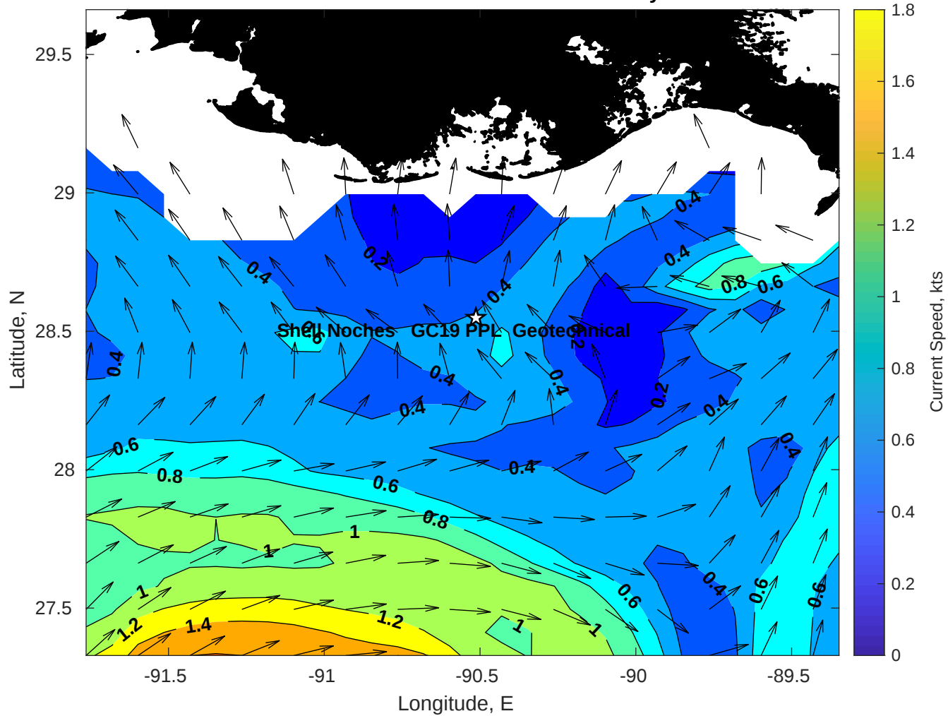
Surface Currents for Shell Noches GC19 PPL Geotechnical at 03-May-2025 00:00:00
