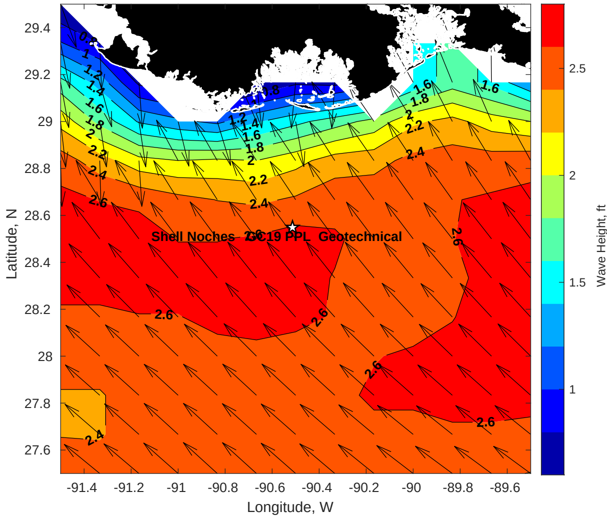
Wave Height (ft) for Shell Noches GC19 PPL Geotechnical at 04-May-2025 09:00:00
