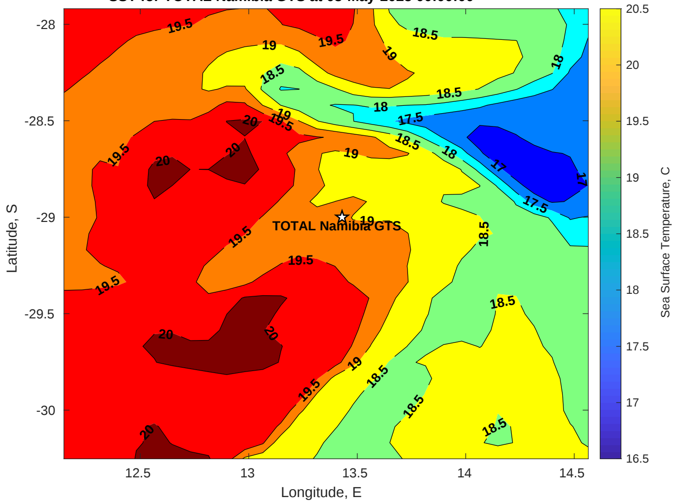
SST for TOTAL Namibia GTS at 03-May-2025 00:00:00
