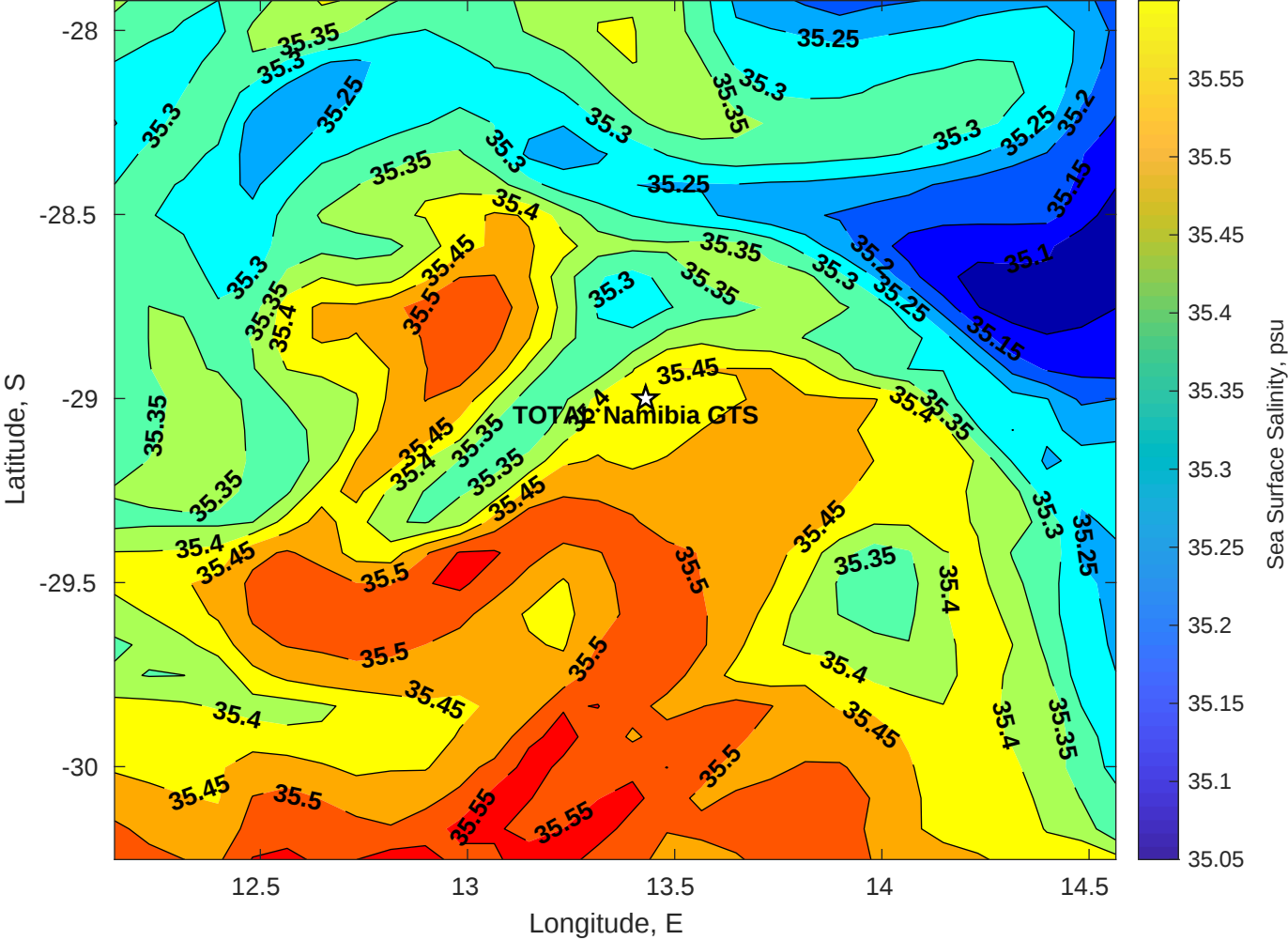
Surface Salinity for TOTAL Namibia GTS at 03-May-2025 00:00:00
