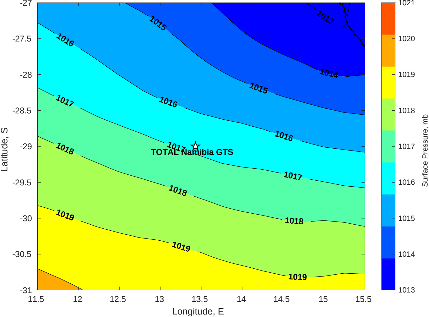
Surface Pressure (mb) for TOTAL Namibia GTS at 04-May-2025 00:00:00
