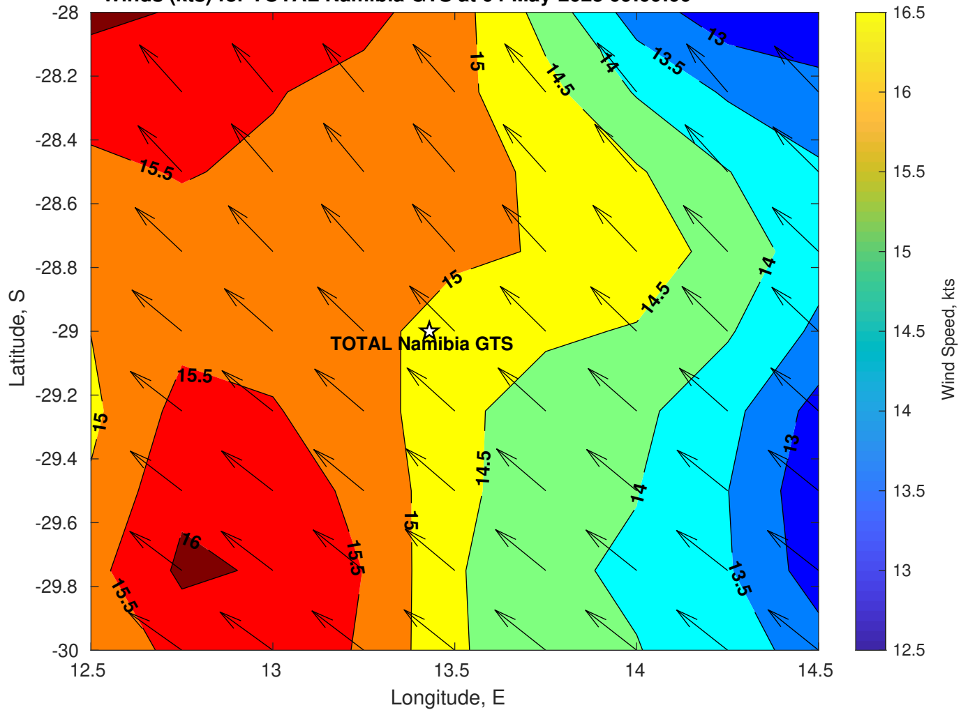
Winds (kts) for TOTAL Namibia GTS at 04-May-2025 09:00:00
