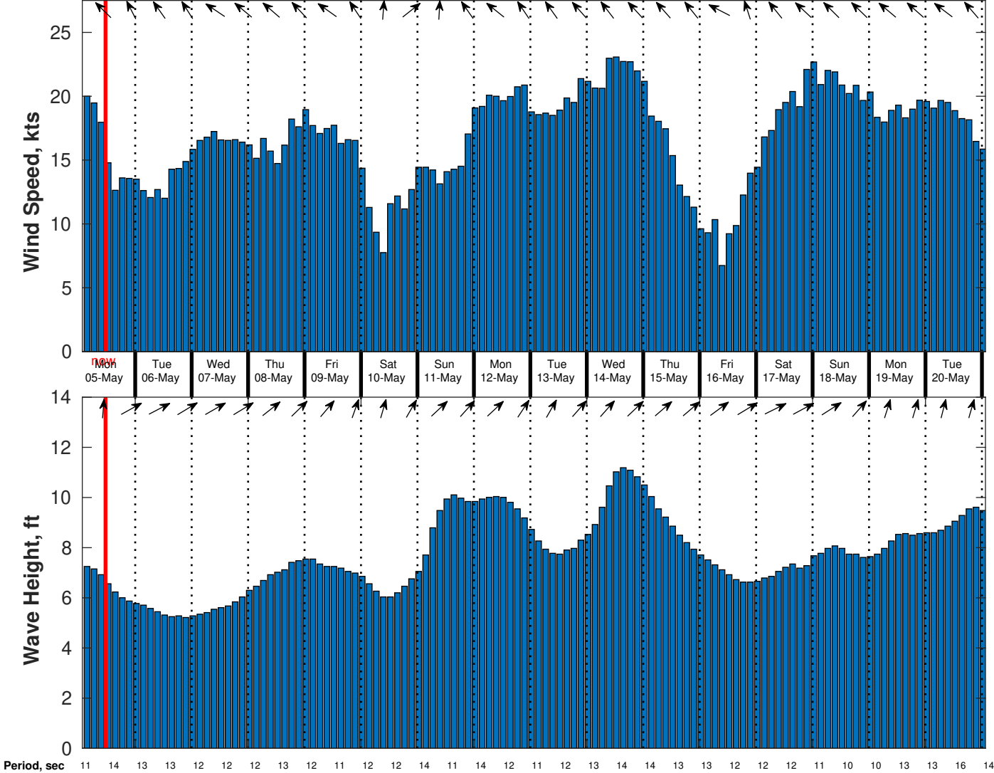
Wind & Wave Forecast for TOTAL Namibia GTS from 04-May-2025 02:00:00 to 20-May-2025 02:00:00
