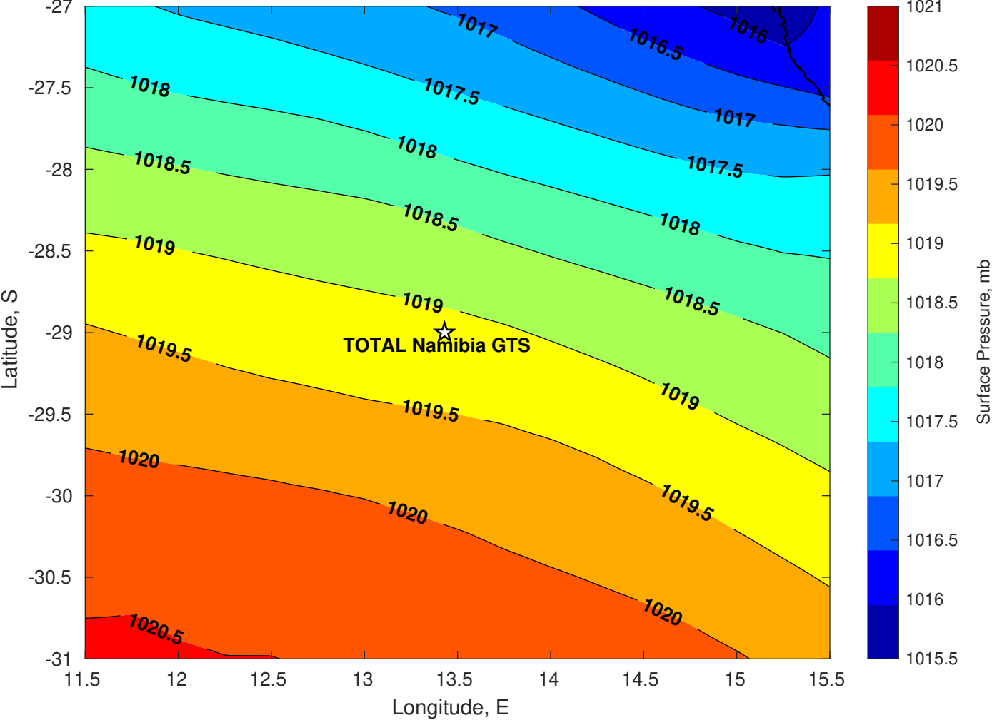
Surface Pressure (mb) for TOTAL Namibia GTS at 06-May-2025 00:00:00
