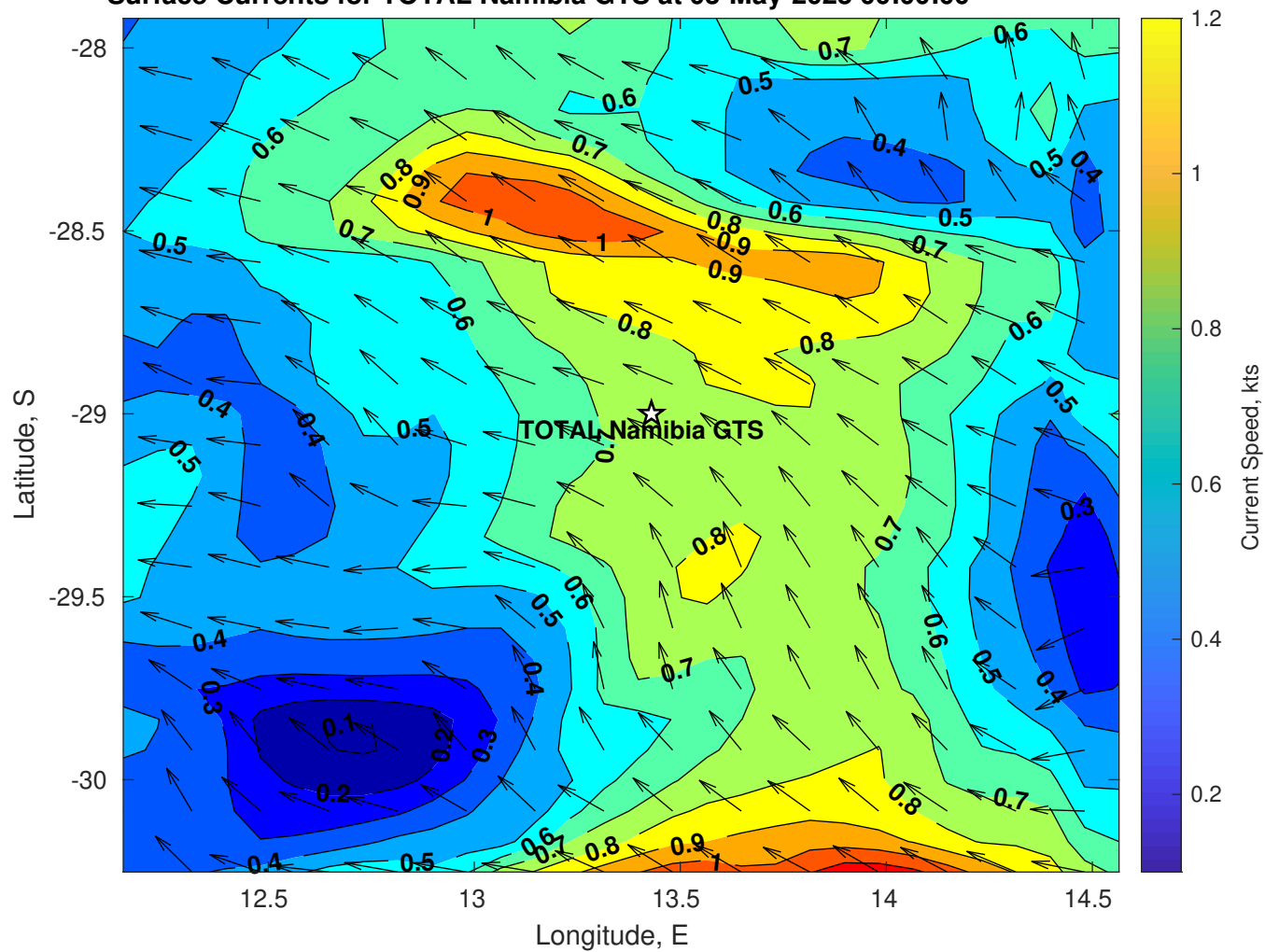
Surface Currents for TOTAL Namibia GTS at 03-May-2025 00:00:00
