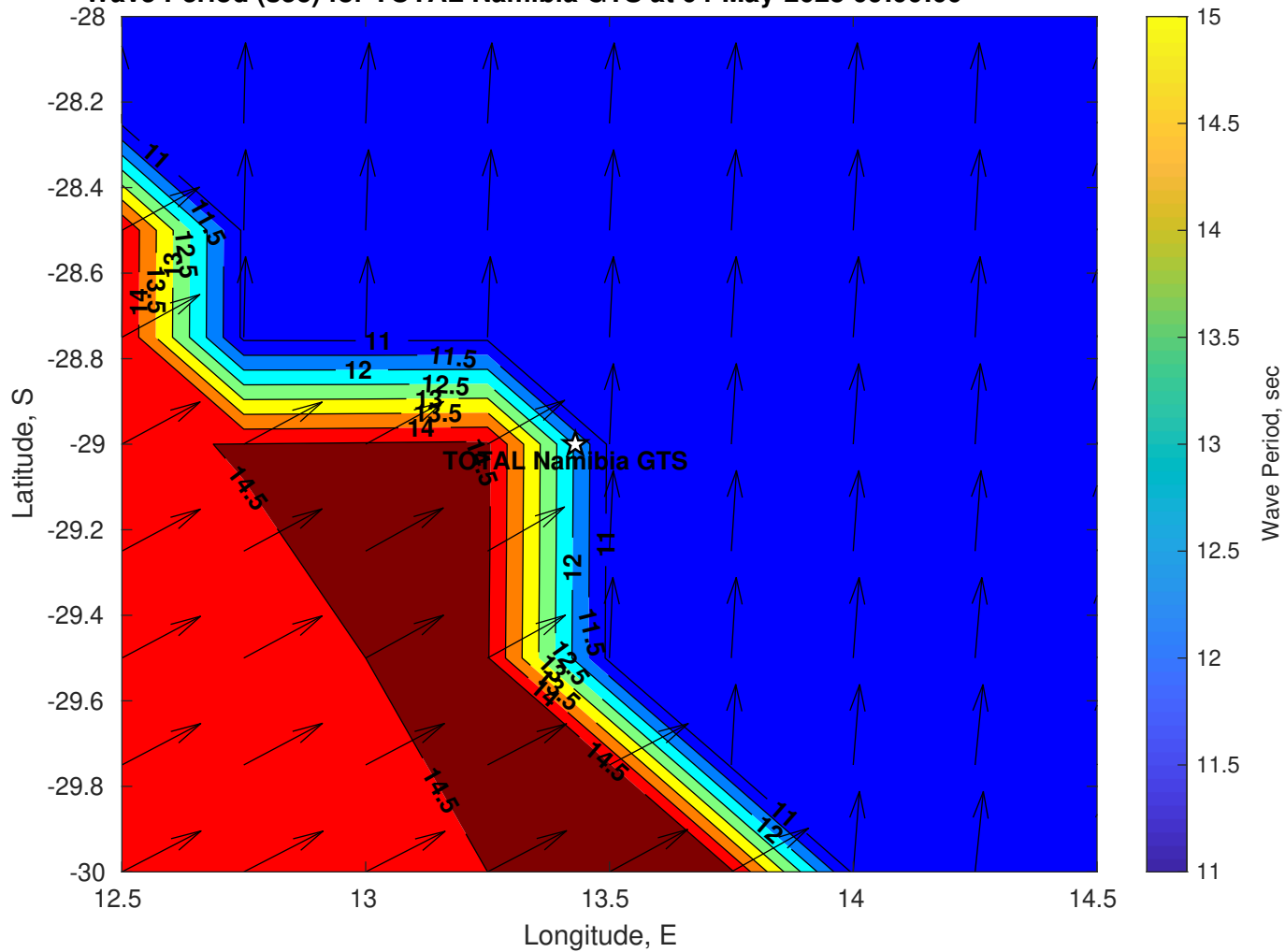
Wave Period (sec) for TOTAL Namibia GTS at 04-May-2025 09:00:00
