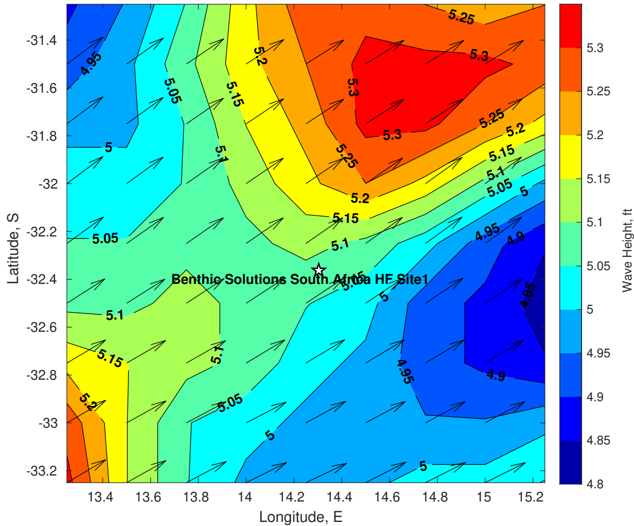
Wave Height (ft) for Benthic Solutions South Africa HF Site1 at 05-May-2025 09:00:00
