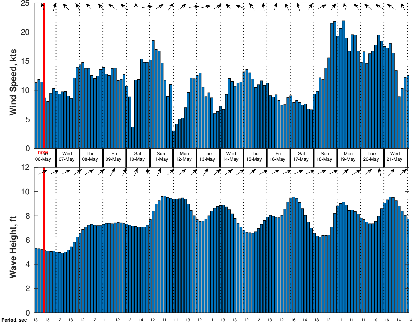
Wind & Wave Forecast for Benthic Solutions South Africa HF Site1 from 05-May-2025 02:00:00 to 21-May-2025 02:00:00
