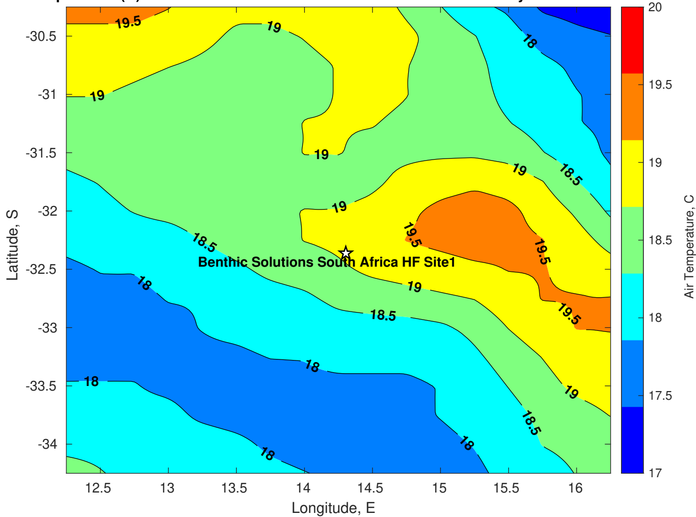
Air Temperature (C) for Benthic Solutions South Africa HF Site1 at 05-May-2025
