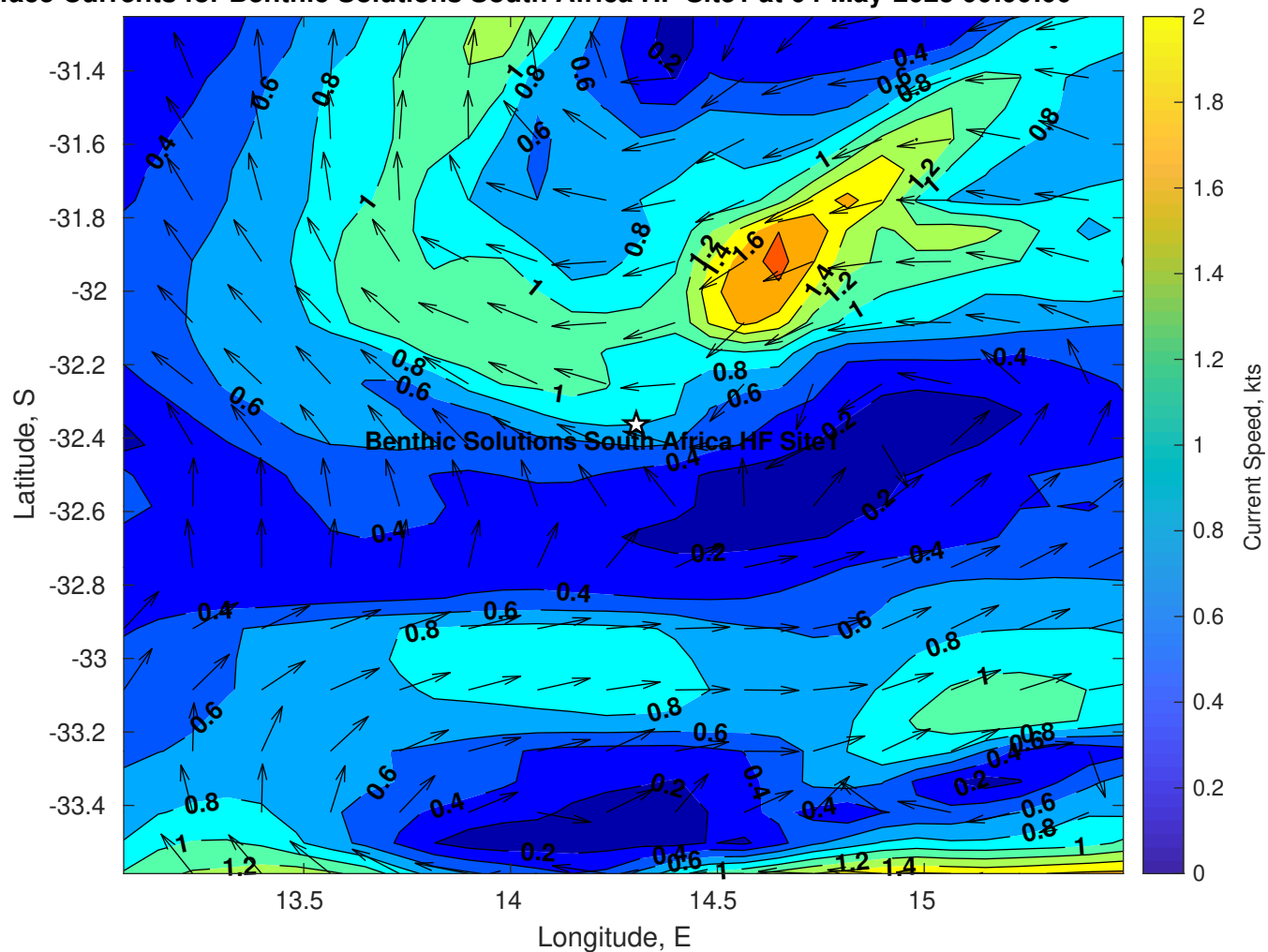
Surface Currents for Benthic Solutions South Africa HF Site1 at 04-May-2025 00:00:00
