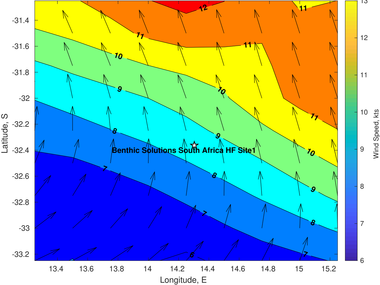
Winds (kts) for Benthic Solutions South Africa HF Site1 at 05-May-2025 09:00:00
