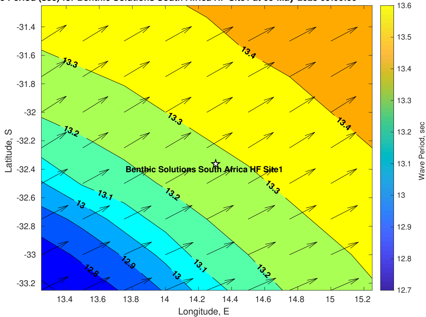
Wave Period (sec) for Benthic Solutions South Africa HF Site1 at 05-May-2025 09:00:00
