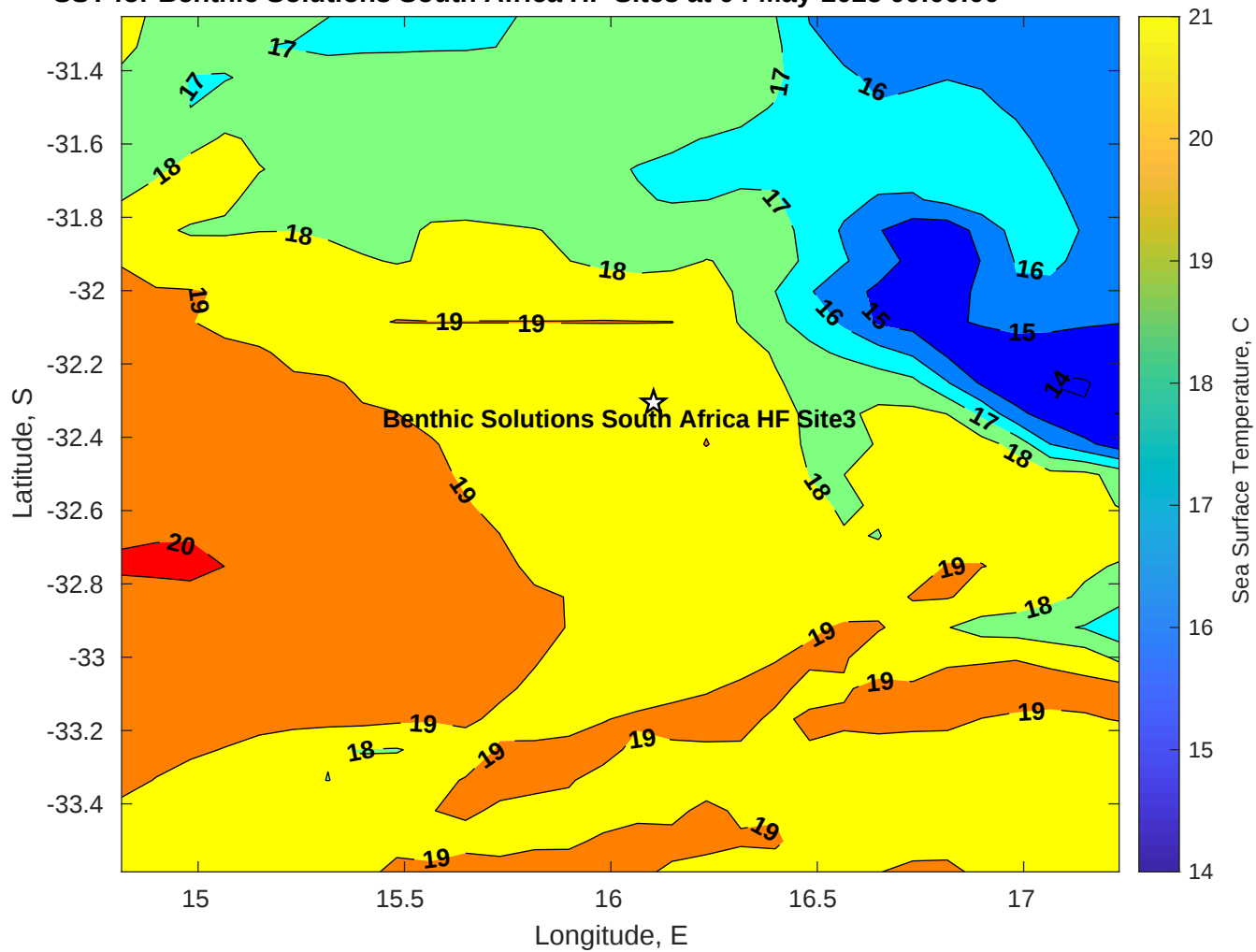
SST for Benthic Solutions South Africa HF Site3 at 04-May-2025 00:00:00
