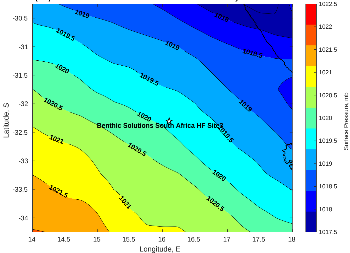
Surface Pressure (mb) for Benthic Solutions South Africa HF Site3 at 07-May-2025 00:00:00
