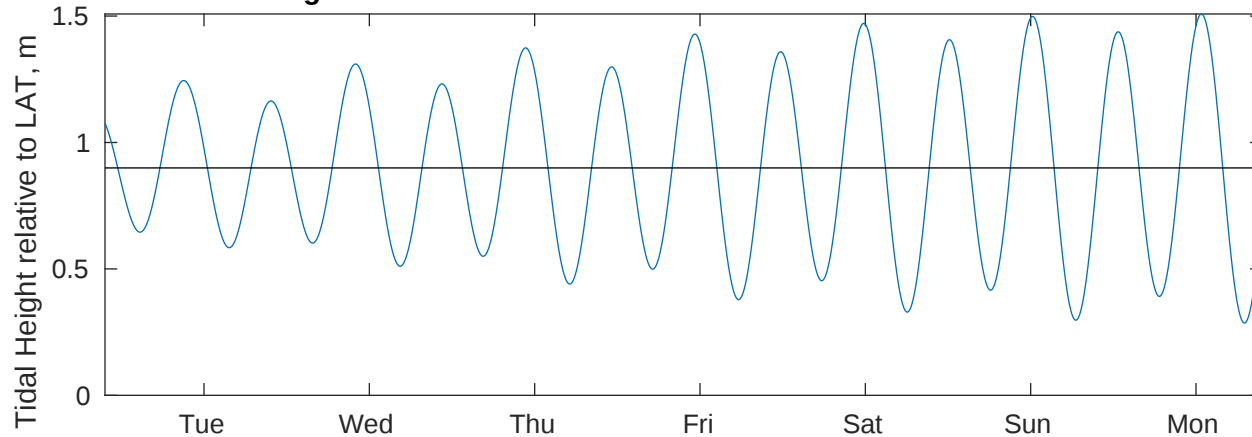
Tidal Currents and Heights for Benthic Solutions South Africa HF Site3 at 20250505
