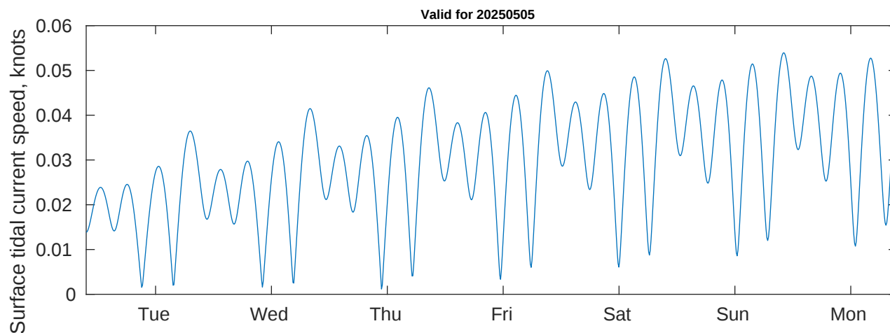
Tidal Currents and Heights for Benthic Solutions South Africa HF Site3 at 20250505
