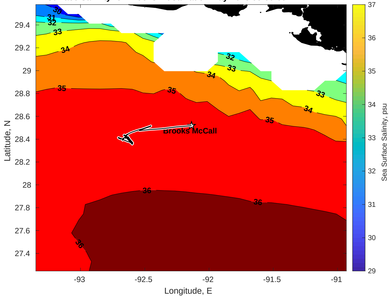
Surface Salinity for Brooks McCall at 04-May-2025 00:00:00
