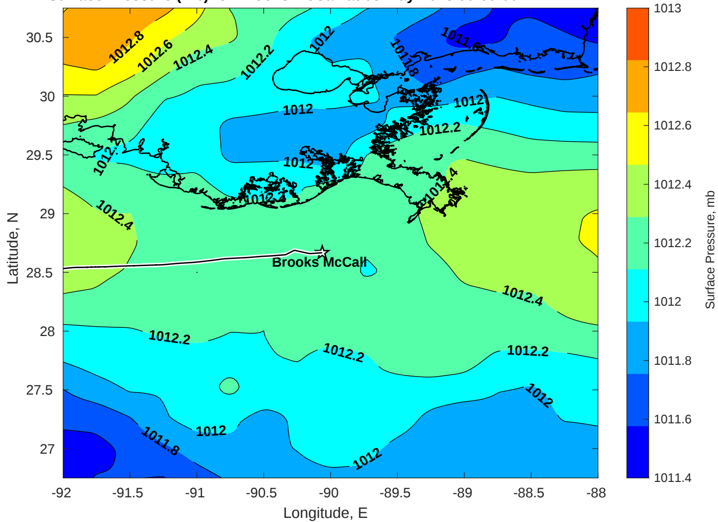
Surface Pressure (mb) for Brooks McCall at 05-May-2025 00:00:00
