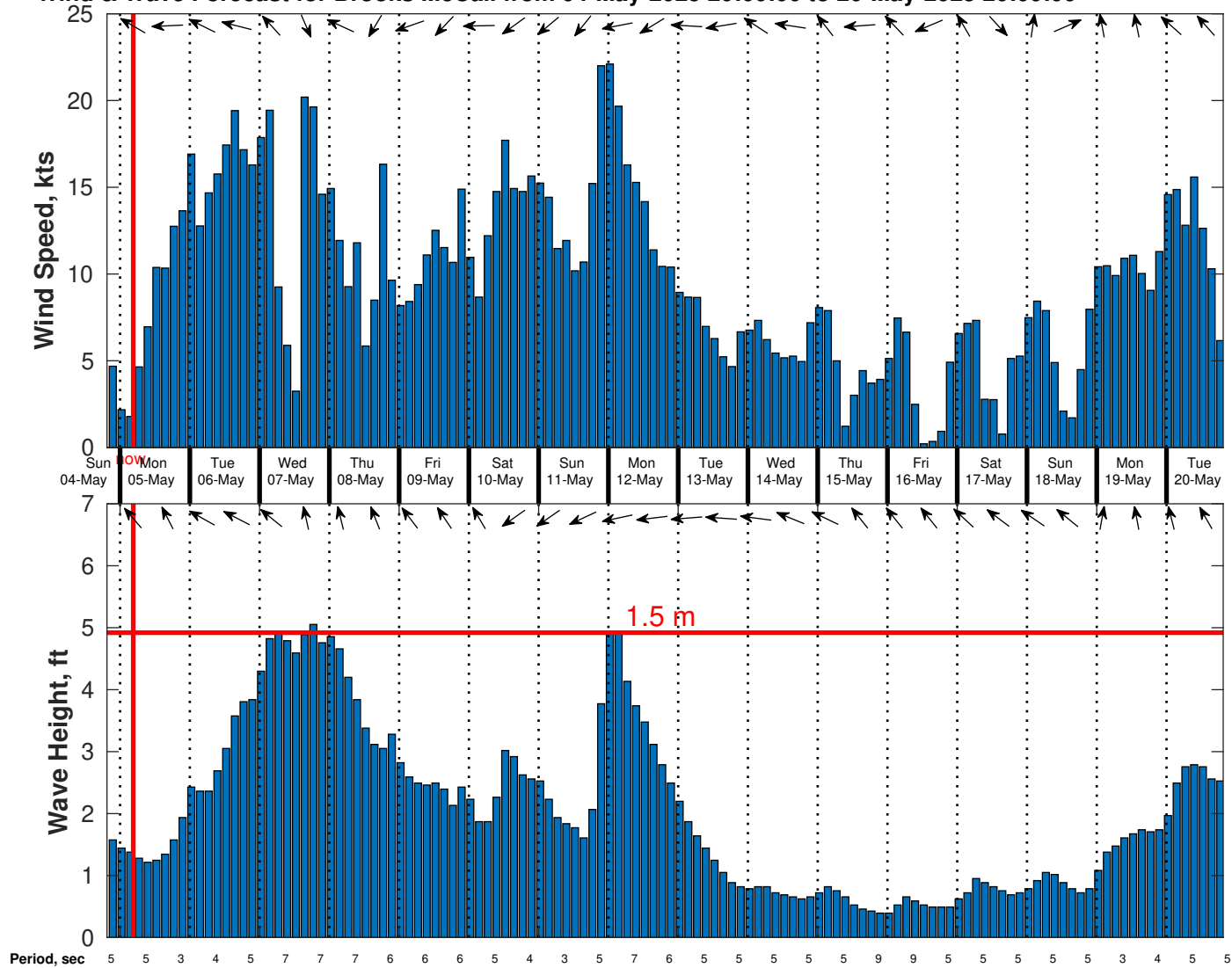
Wind & Wave Forecast for Brooks McCall from 04-May-2025 20:00:00 to 20-May-2025 20:00:00
