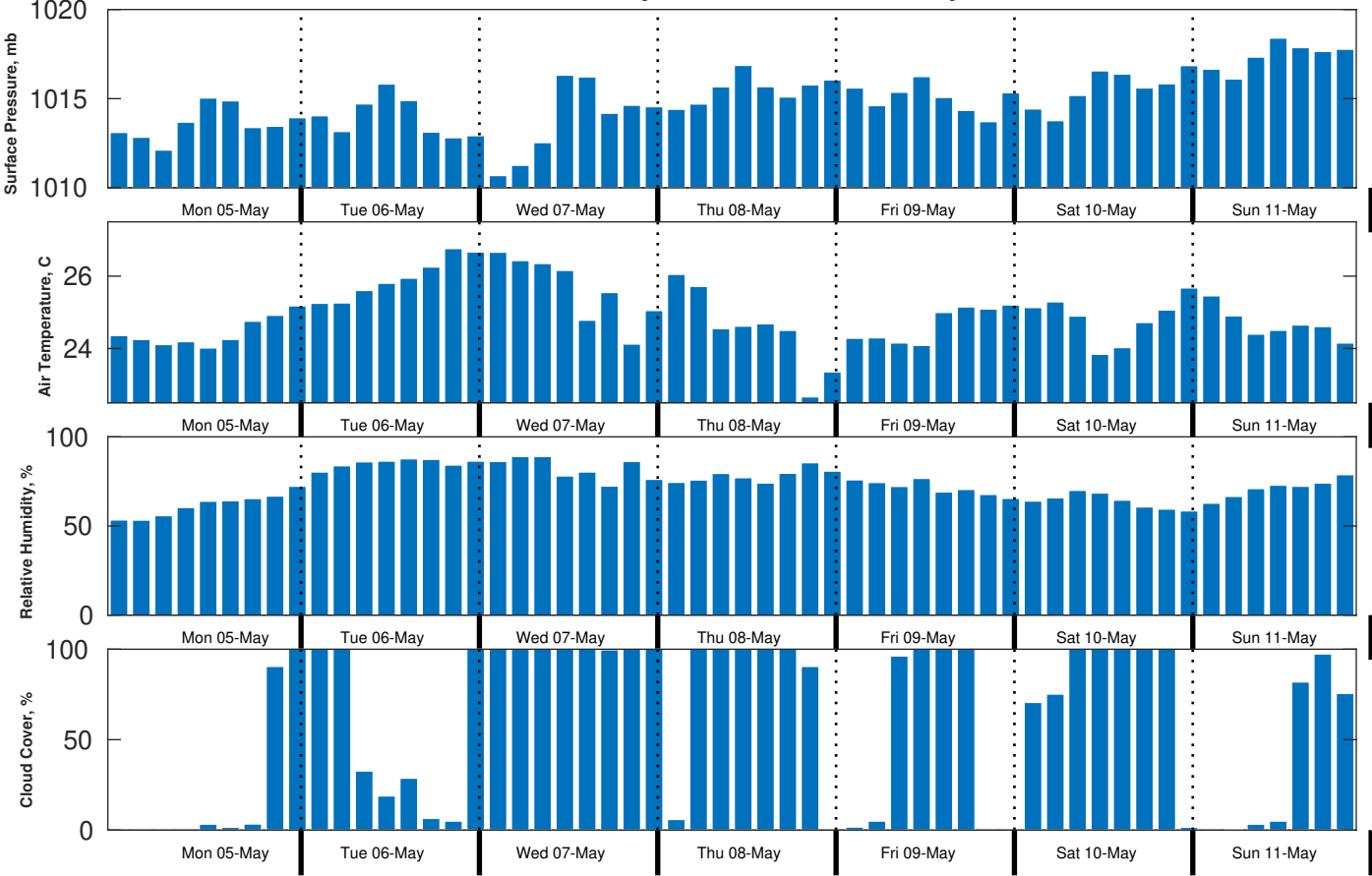
Met Forecast for Brooks McCall from 05-May-2025 00:00:00 to 12-May-2025 00:00:00
