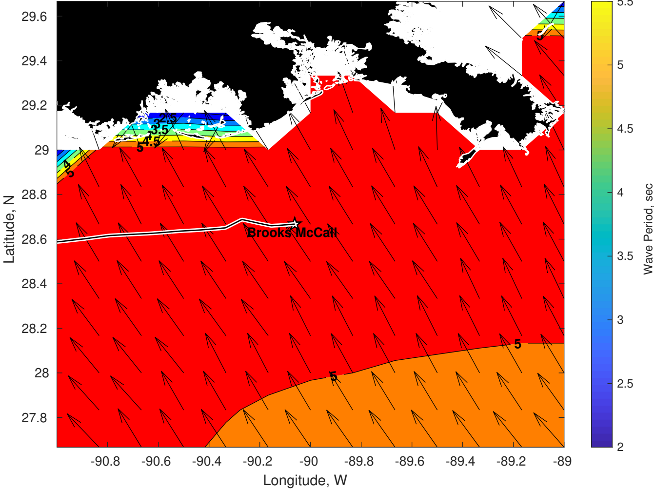
Wave Period (sec) for Brooks McCall at 05-May-2025 09:00:00
