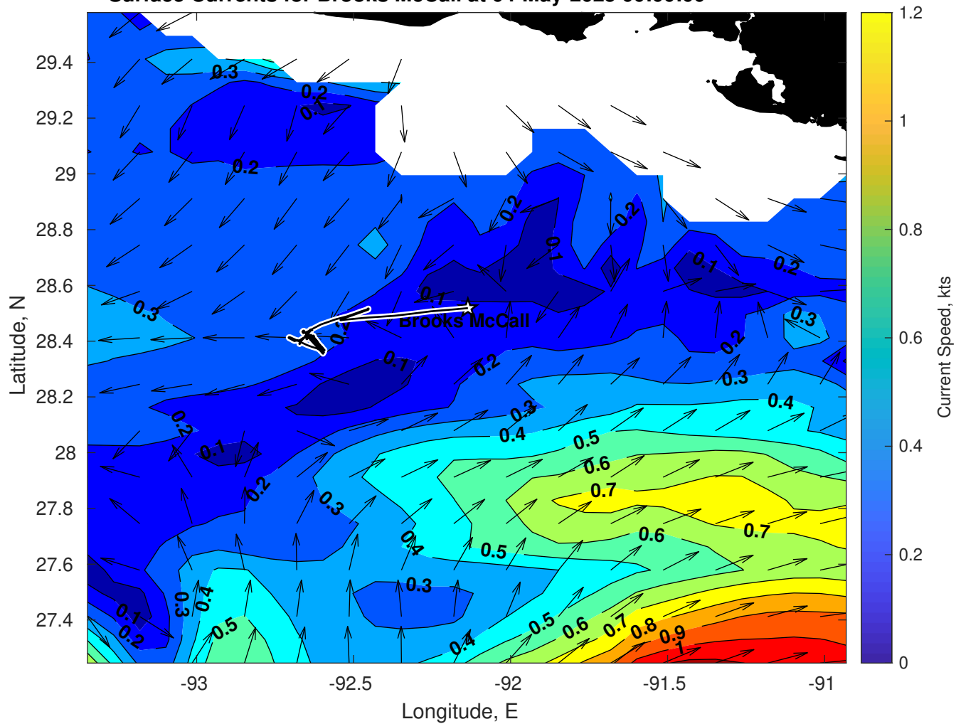
Surface Currents for Brooks McCall at 04-May-2025 00:00:00
