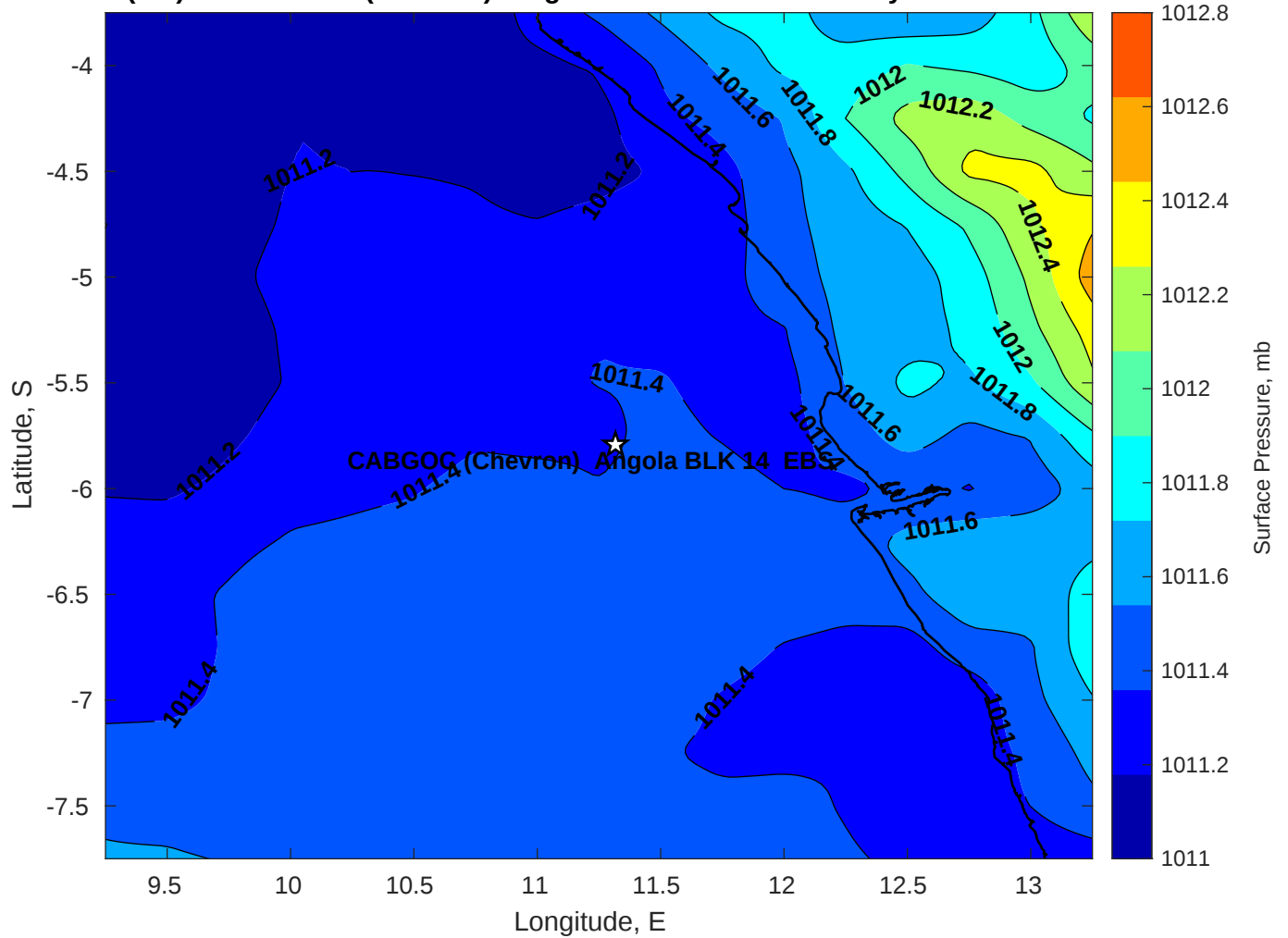
Surface Pressure (mb) for CABGOC (Chevron) Angola BLK 14 EBS at 05-May-2025 00:00:00
