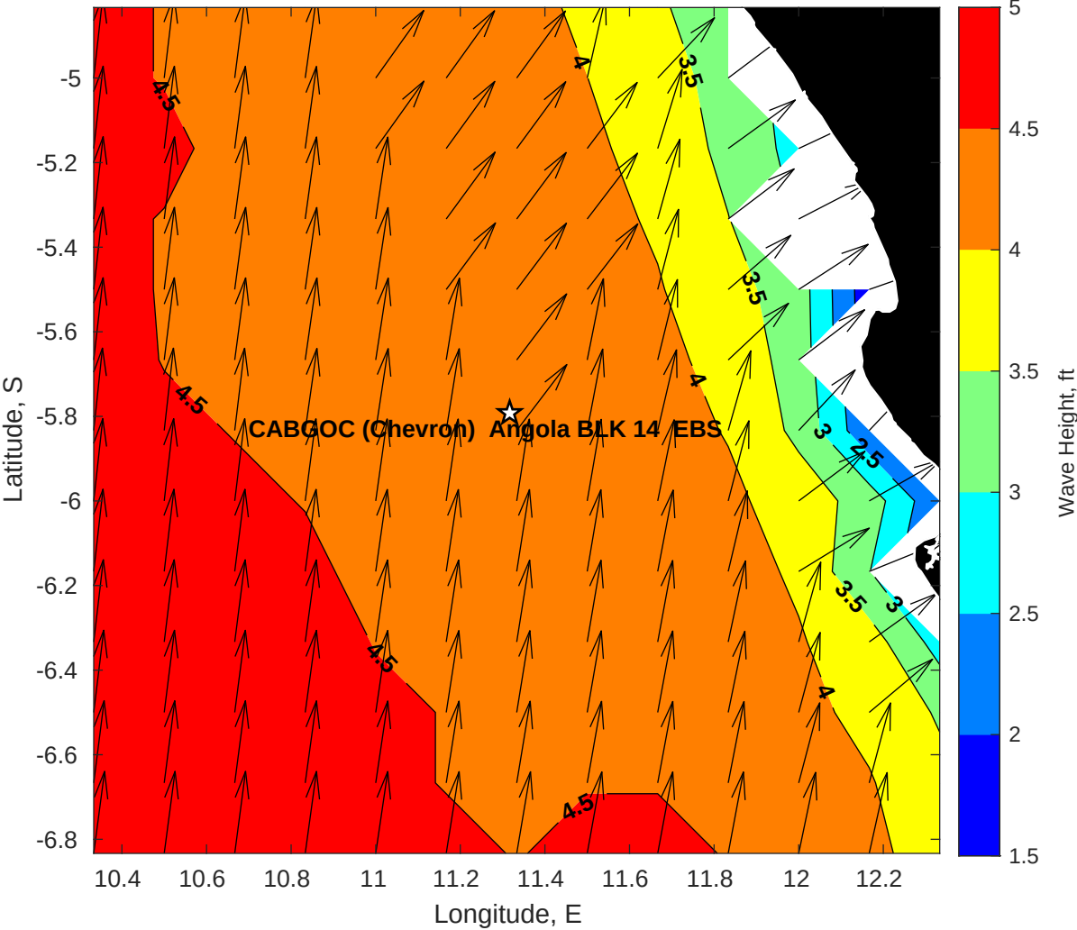
Wave Height (ft) for CABGOC (Chevron) Angola BLK 14 EBS at 05-May-2025 09:00:00
