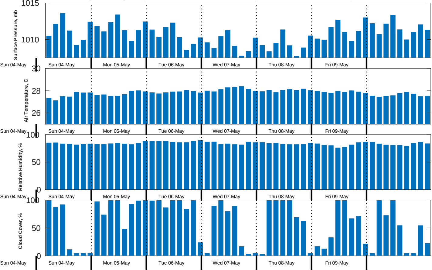
Met Forecast for CABGOC (Chevron) Angola BLK 14 EBS from 05-May-2025 00:00:00 to 12-May-2025 00:00:00
