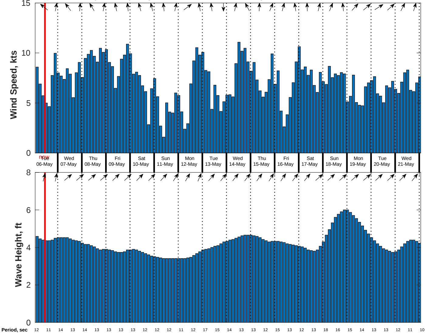
Wind & Wave Forecast for CABGOC (Chevron) Angola BLK 14 EBS from 05-May-2025 02:00:00 to 21-May-2025 02:00:00
