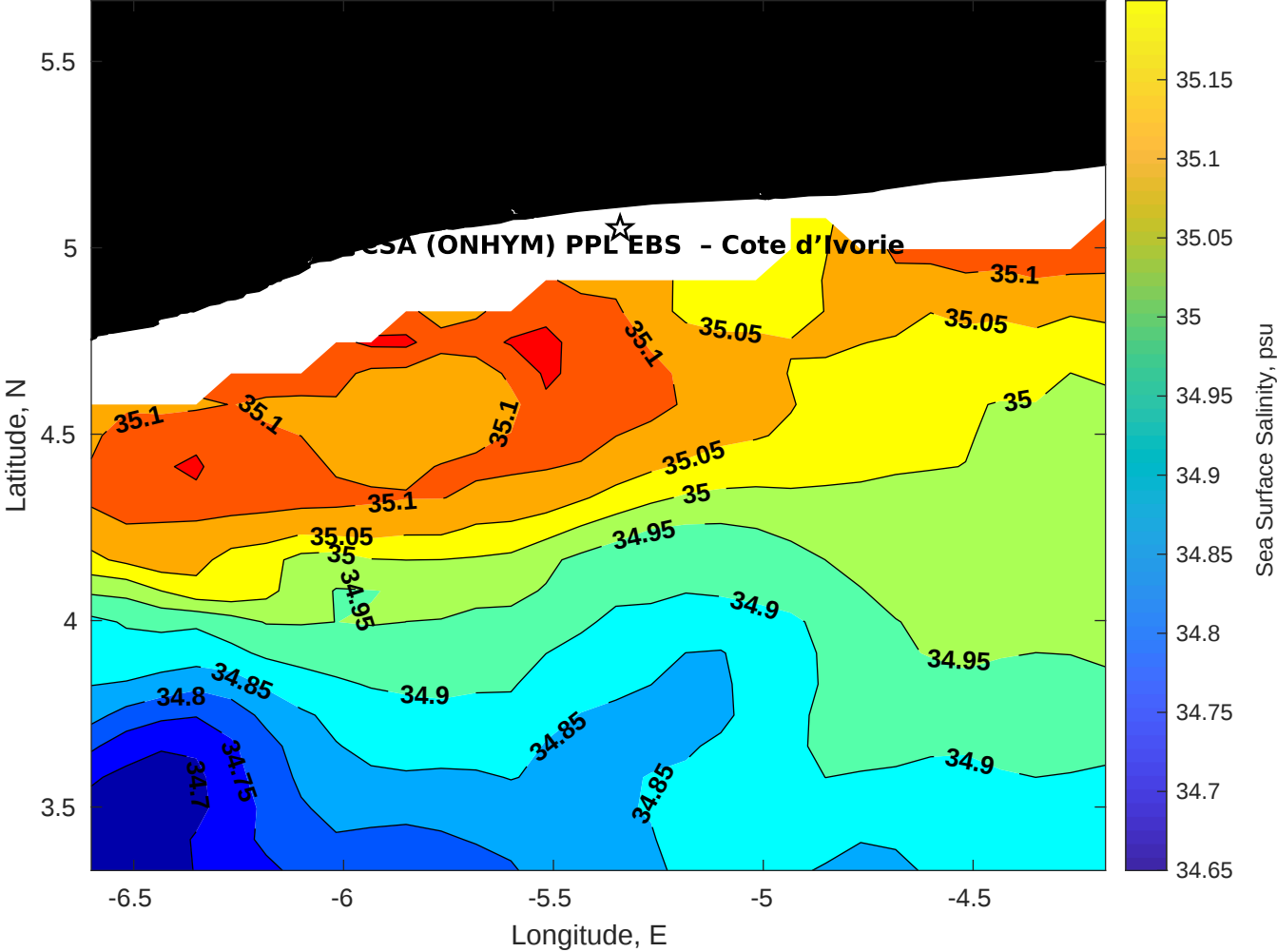
Surface Salinity for CSA (ONHYM) PPL EBS - Cote d'Ivoire at 04-May-2025 00:00:00
