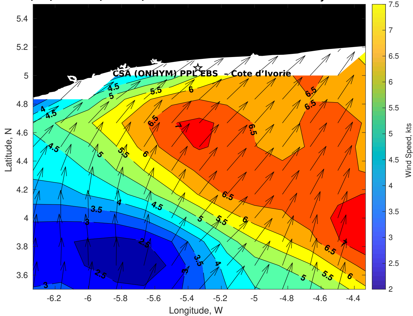
Winds (kts) for CSA (ONHYM) PPL EBS - Cote d'Ivoire at 05-May-2025 09:00:00
