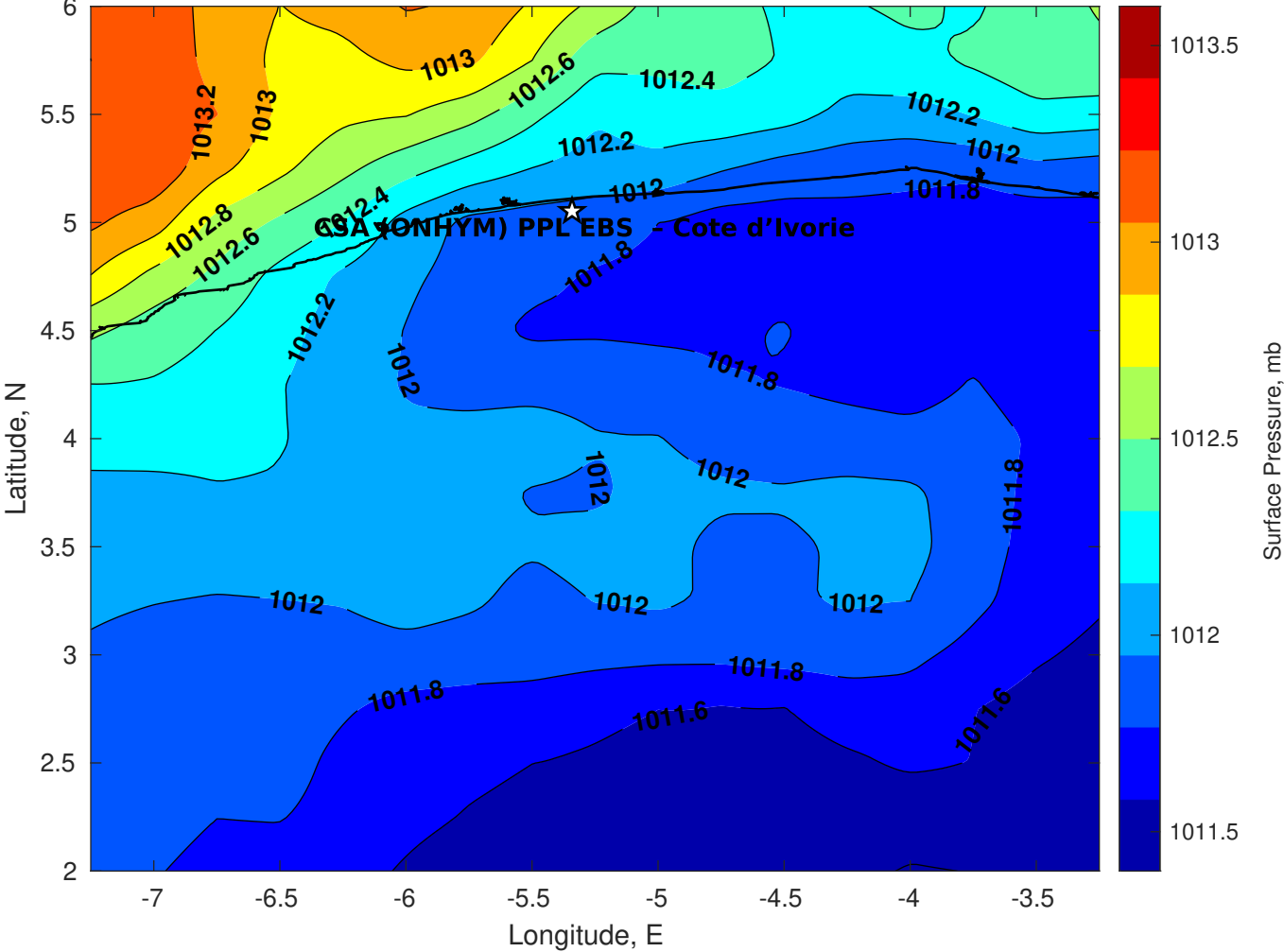
Surface Pressure (mb) for CSA (ONHYM) PPL EBS - Cote d'Ivoire at 07-May-2025 00:00:00
