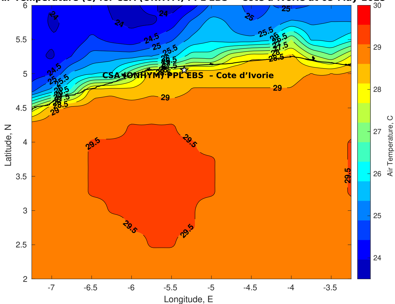
Air Temperature (C) for CSA (ONHYM) PPL EBS - Cote d'Ivoire at 05-May-2025
