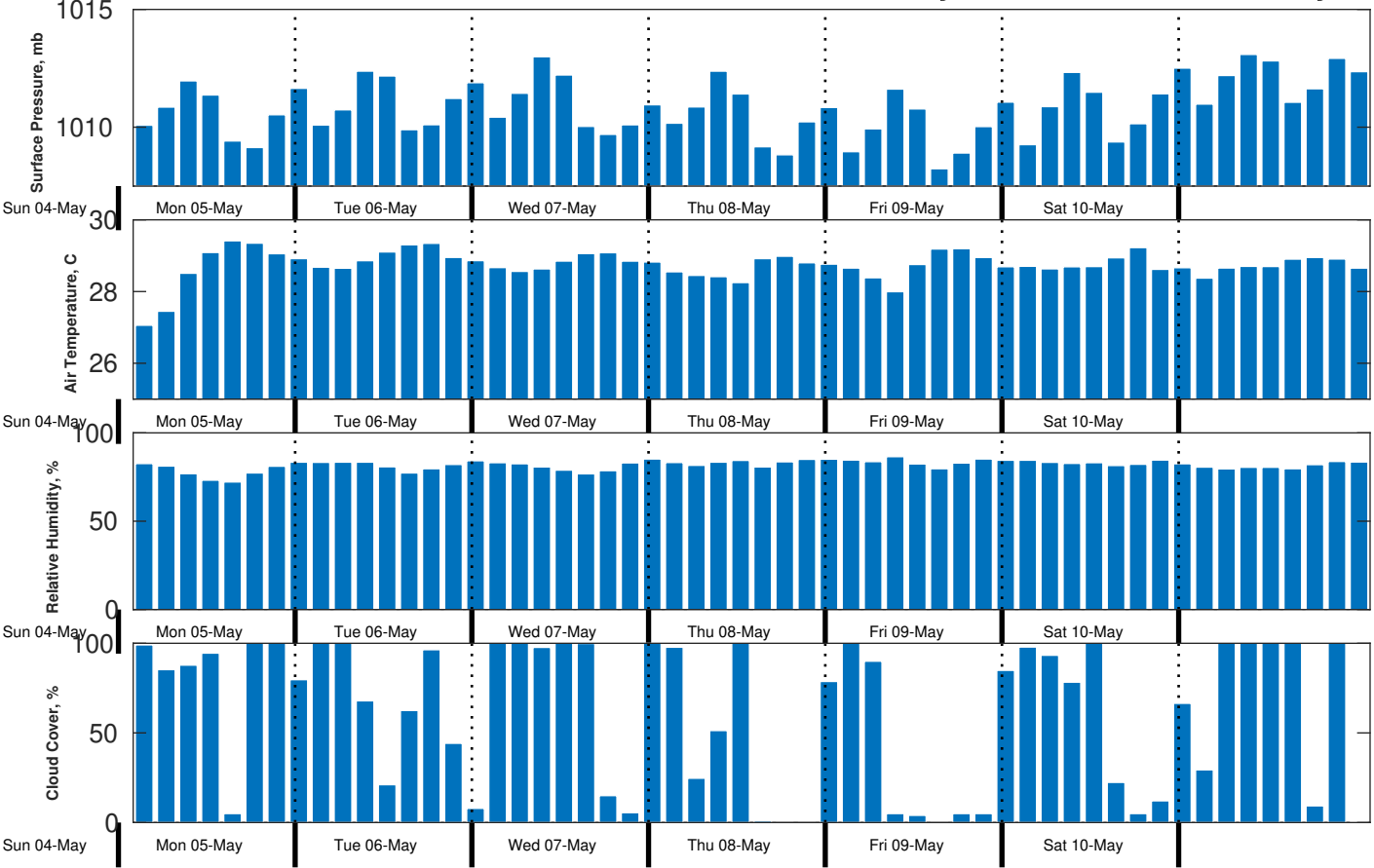
Met Forecast for CSA (ONHYM) PPL EBS - Cote d'Ivoire from 05-May-2025 00:00:00 to 12-May-2025 00:00:00
