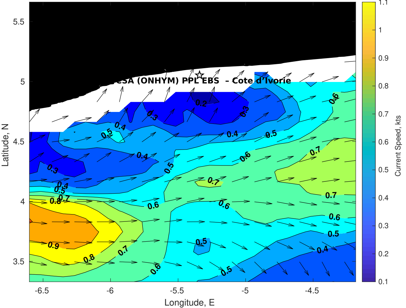
Surface Currents for CSA (ONHYM) PPL EBS - Cote d'Ivoire at 04-May-2025 00:00:00
