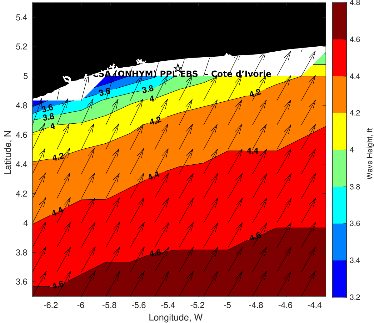
Wave Height (ft) for CSA (ONHYM) PPL EBS - Cote d'Ivoire at 05-May-2025 09:00:00
