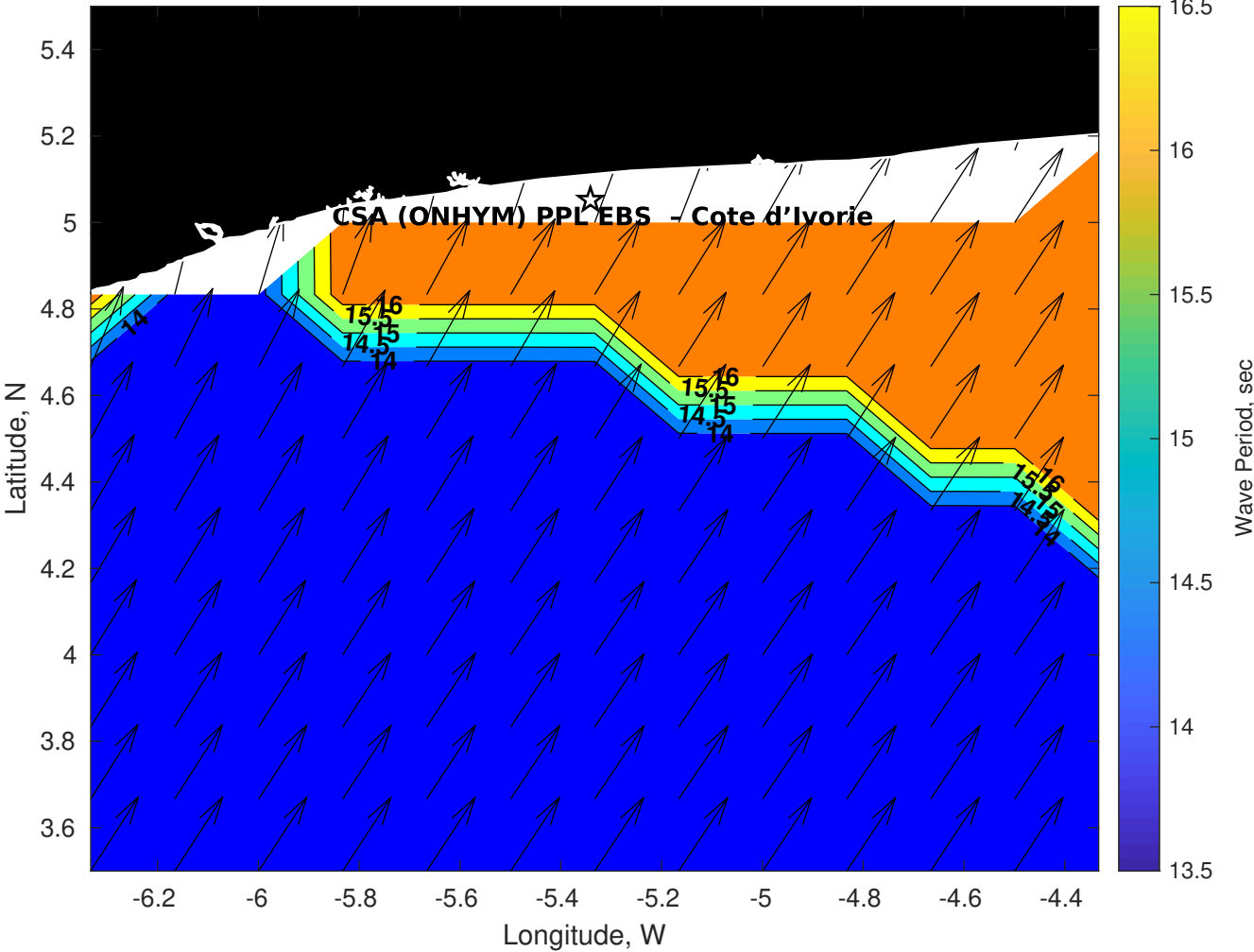
Wave Period (sec) for CSA (ONHYM) PPL EBS - Cote d'Ivoire at 05-May-2025 09:00:00
