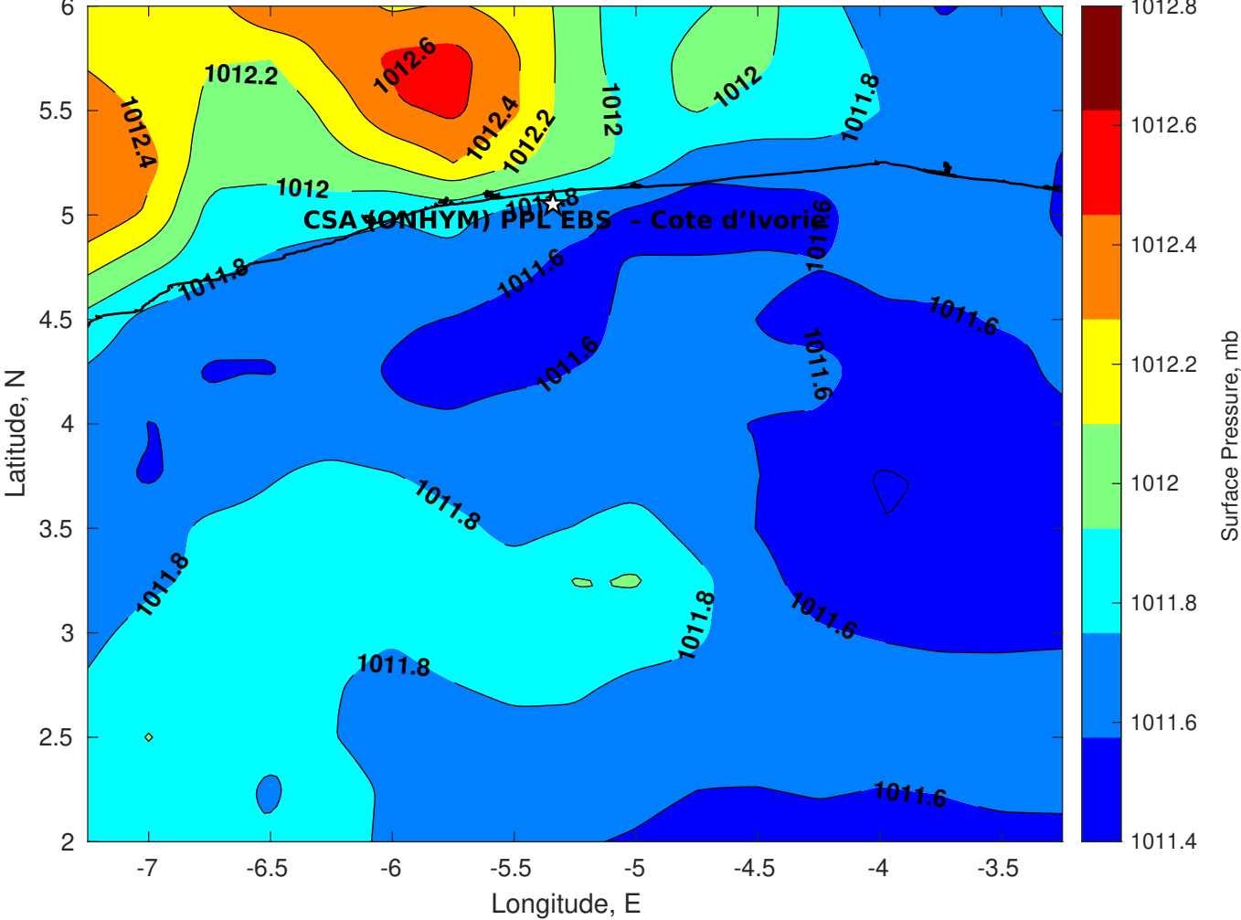
Surface Pressure (mb) for CSA (ONHYM) PPL EBS - Cote d'Ivoire at 05-May-2025 00:00:00
