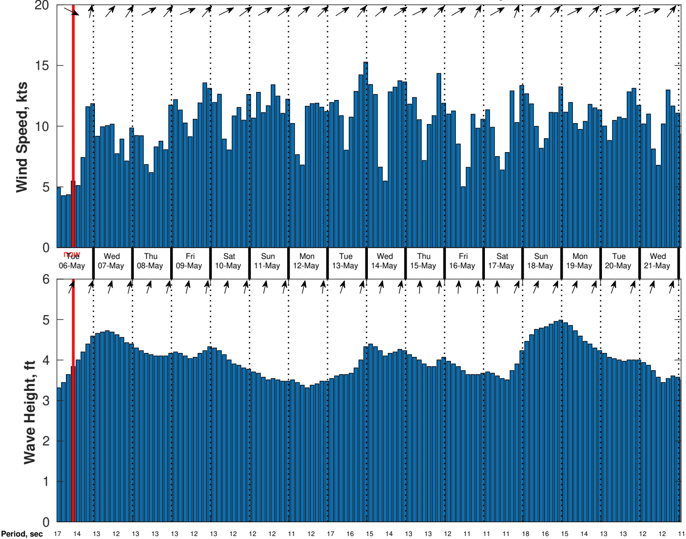
Wind & Wave Forecast for CSA (ONHYM) PPL EBS - Cote d'Ivoire from 05-May-2025 01:00:00 to 21-May-2025 01:00:00
