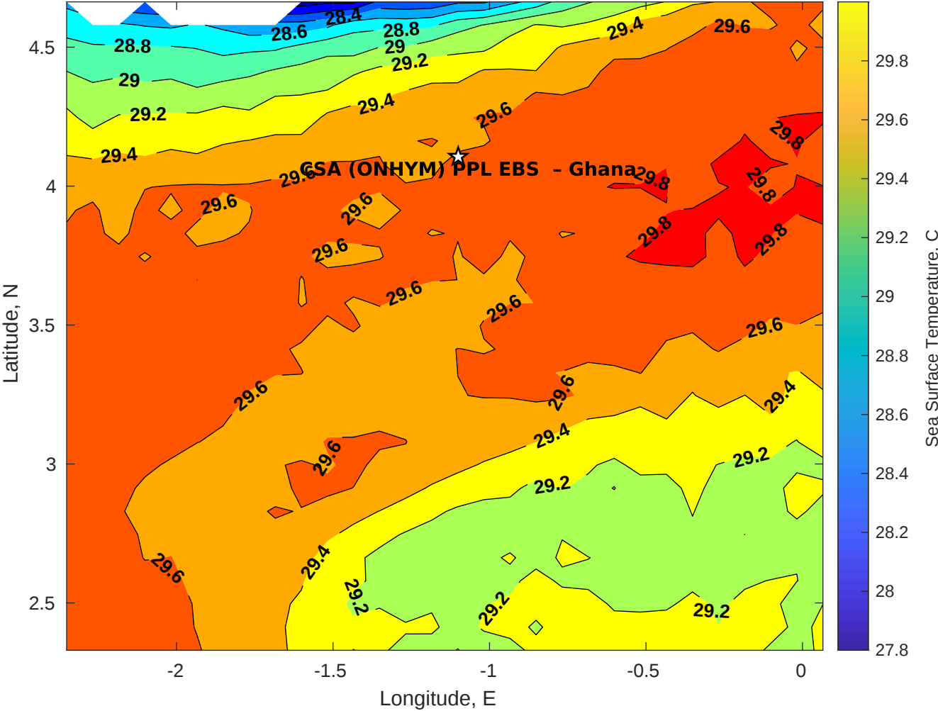
SST for CSA (ONHYM) PPL EBS - Ghana at 04-May-2025 00:00:00
