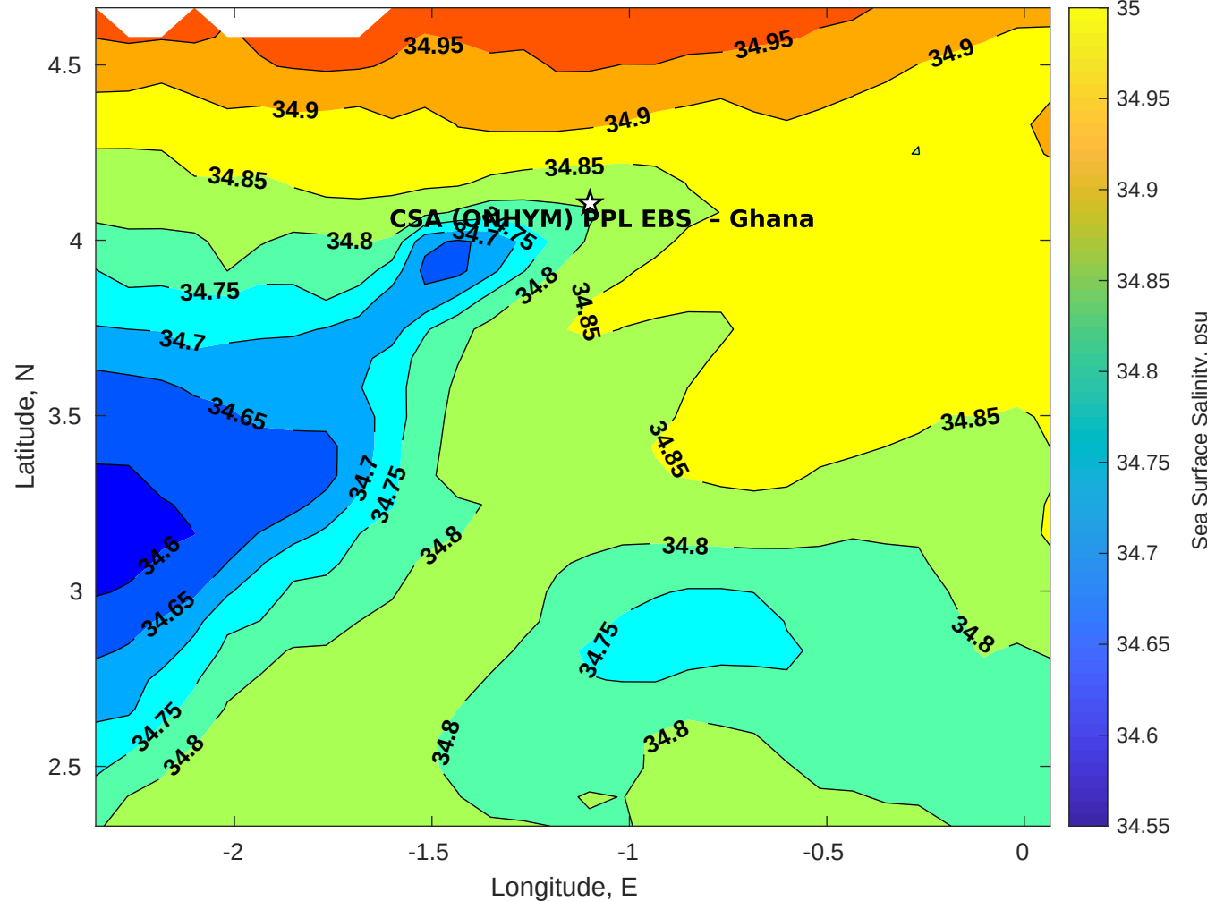
Surface Salinity for CSA (ONHYM) PPL EBS - Ghana at 04-May-2025 00:00:00
