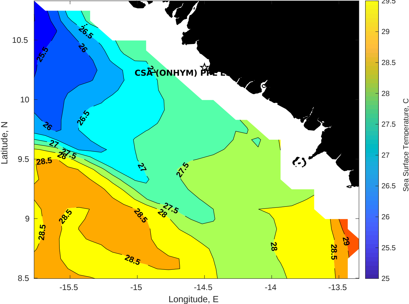
SST for CSA (ONHYM) PPL EBS - Guinea at 04-May-2025 00:00:00
