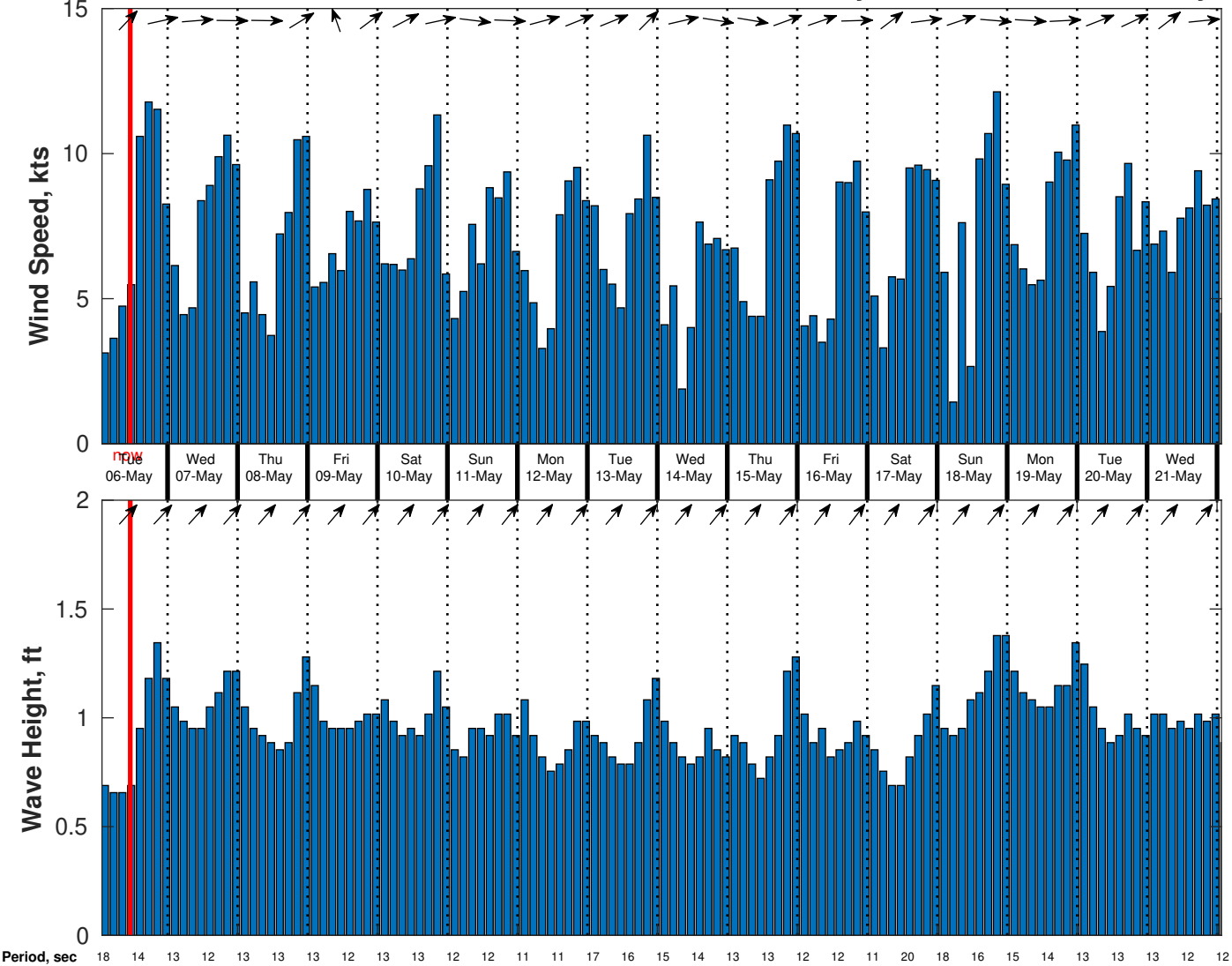
Wind & Wave Forecast for CSA (ONHYM) PPL EBS - Guinea from 05-May-2025 01:00:00 to 21-May-2025 01:00:00
