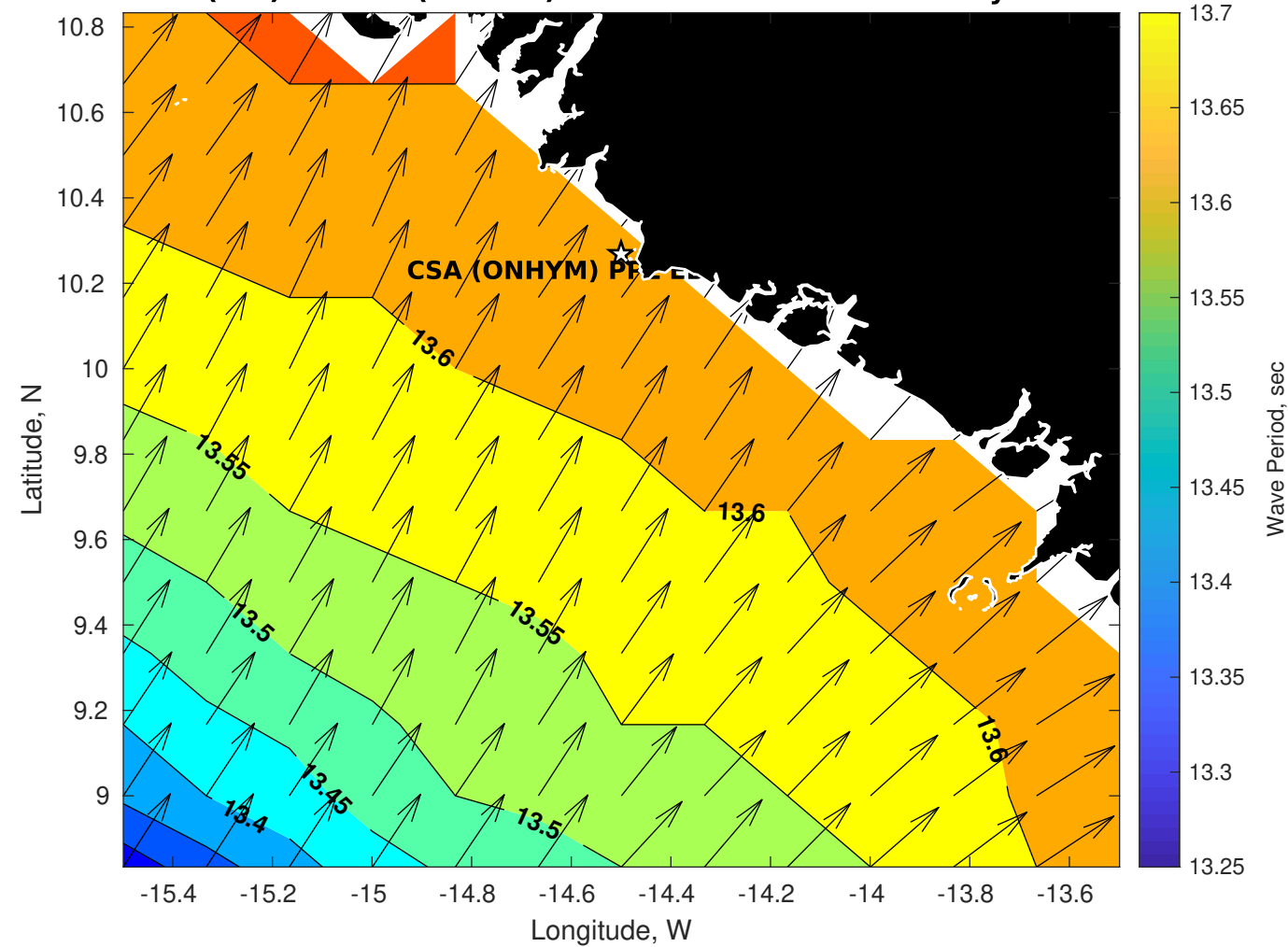
Wave Period (sec) for CSA (ONHYM) PPL EBS - Guinea at 05-May-2025 09:00:00
