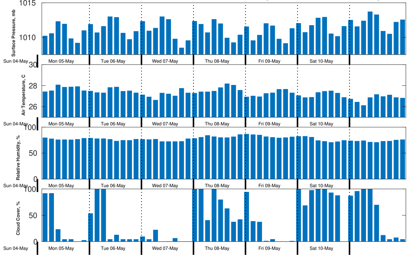
Met Forecast for CSA (ONHYM) PPL EBS - Guinea from 05-May-2025 00:00:00 to 12-May-2025 00:00:00
