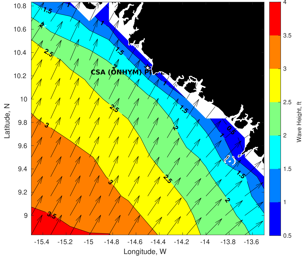
Wave Height (ft) for CSA (ONHYM) PPL EBS - Guinea at 05-May-2025 09:00:00
