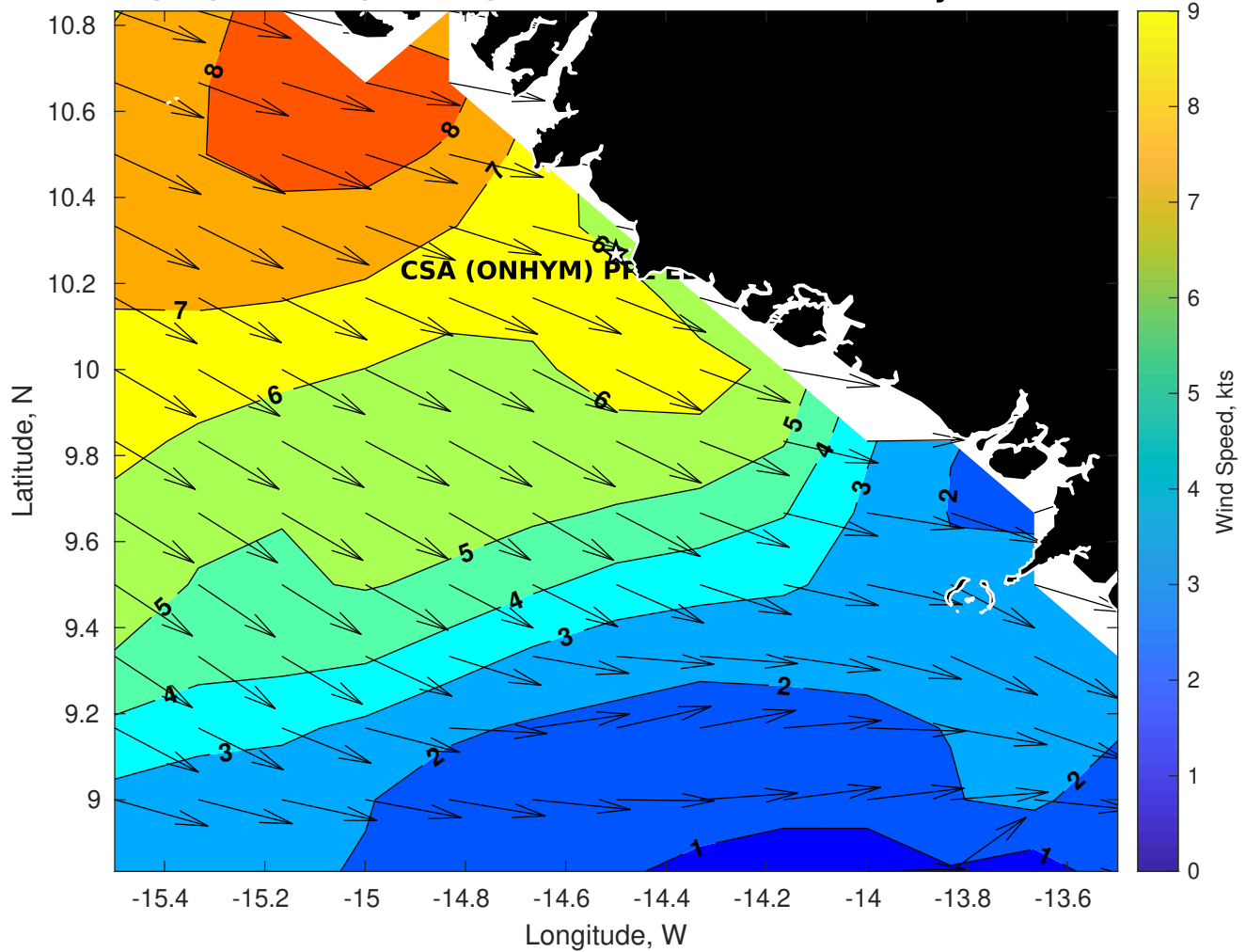
Winds (kts) for CSA (ONHYM) PPL EBS - Guinea at 05-May-2025 09:00:00
