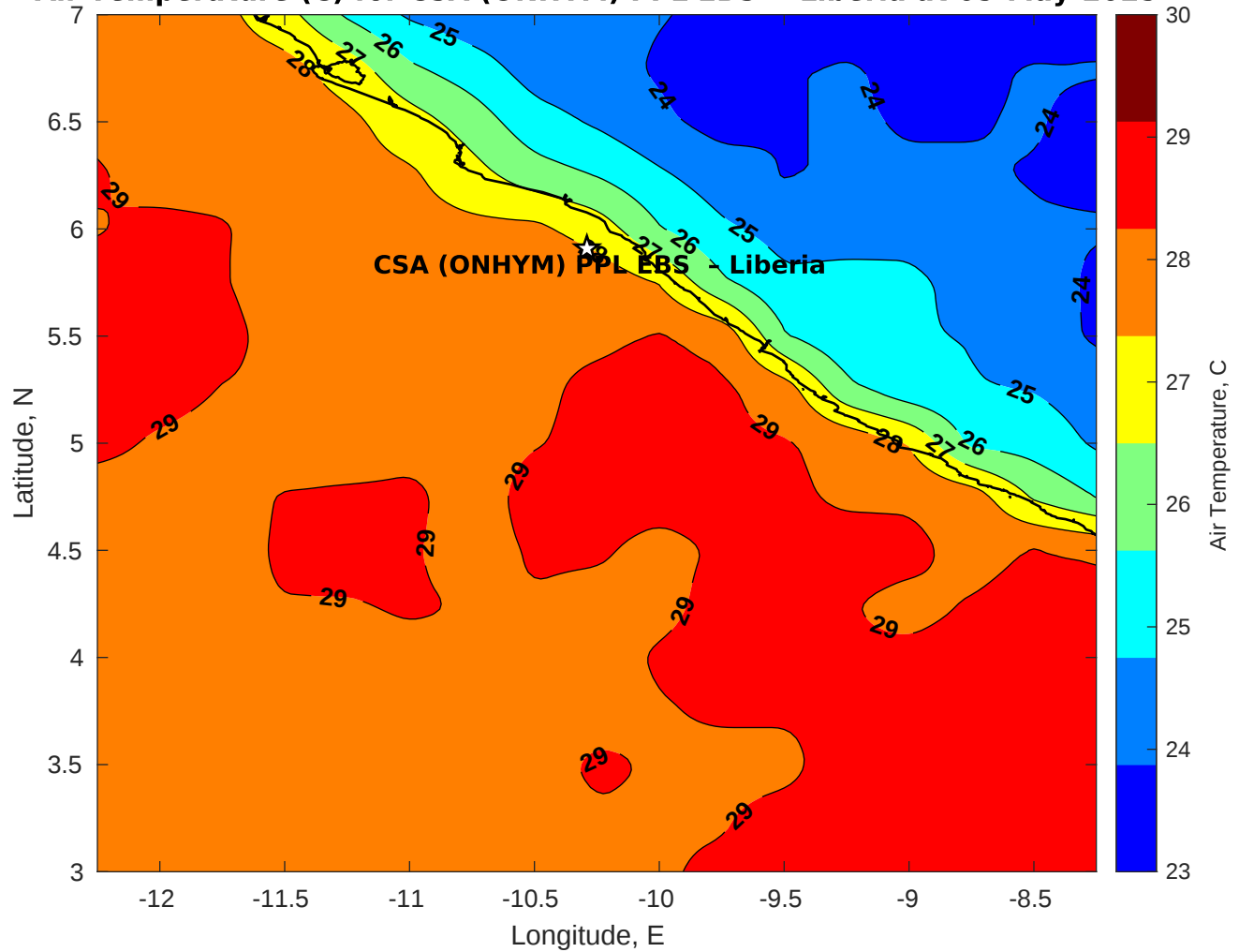
Air Temperature (C) for CSA (ONHYM) PPL EBS - Liberia at 05-May-2025
