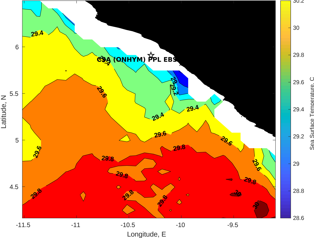
SST for CSA (ONHYM) PPL EBS - Liberia at 04-May-2025 00:00:00
