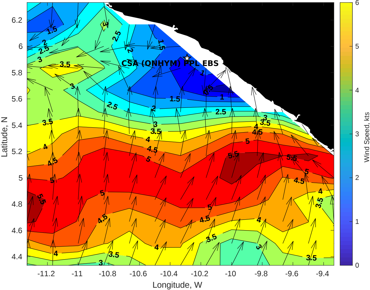
Winds (kts) for CSA (ONHYM) PPL EBS - Liberia at 05-May-2025 09:00:00
