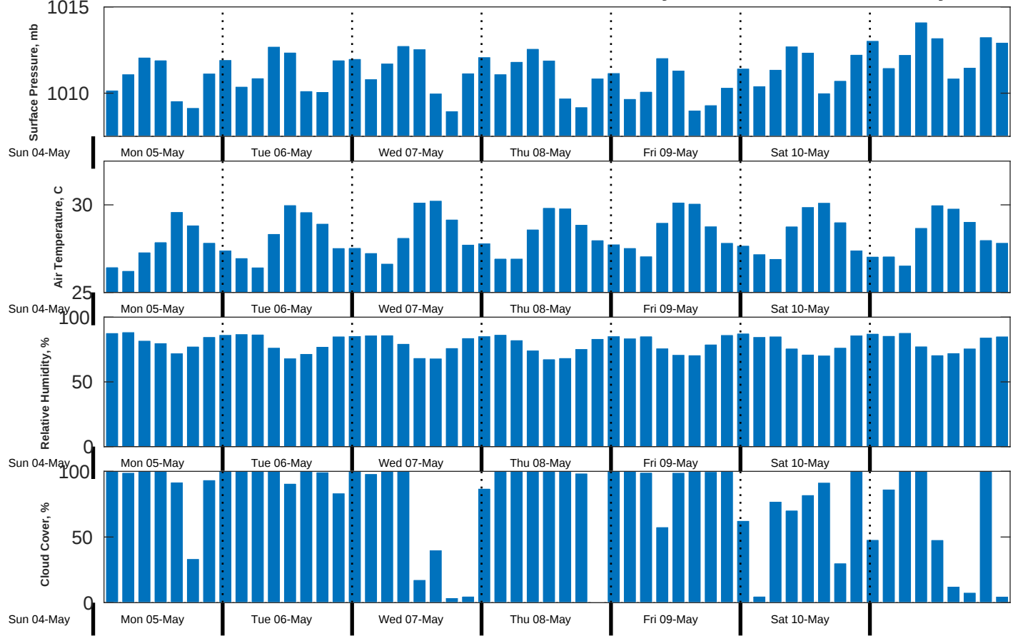
Met Forecast for CSA (ONHYM) PPL EBS - Liberia from 05-May-2025 00:00:00 to 12-May-2025 00:00:00
