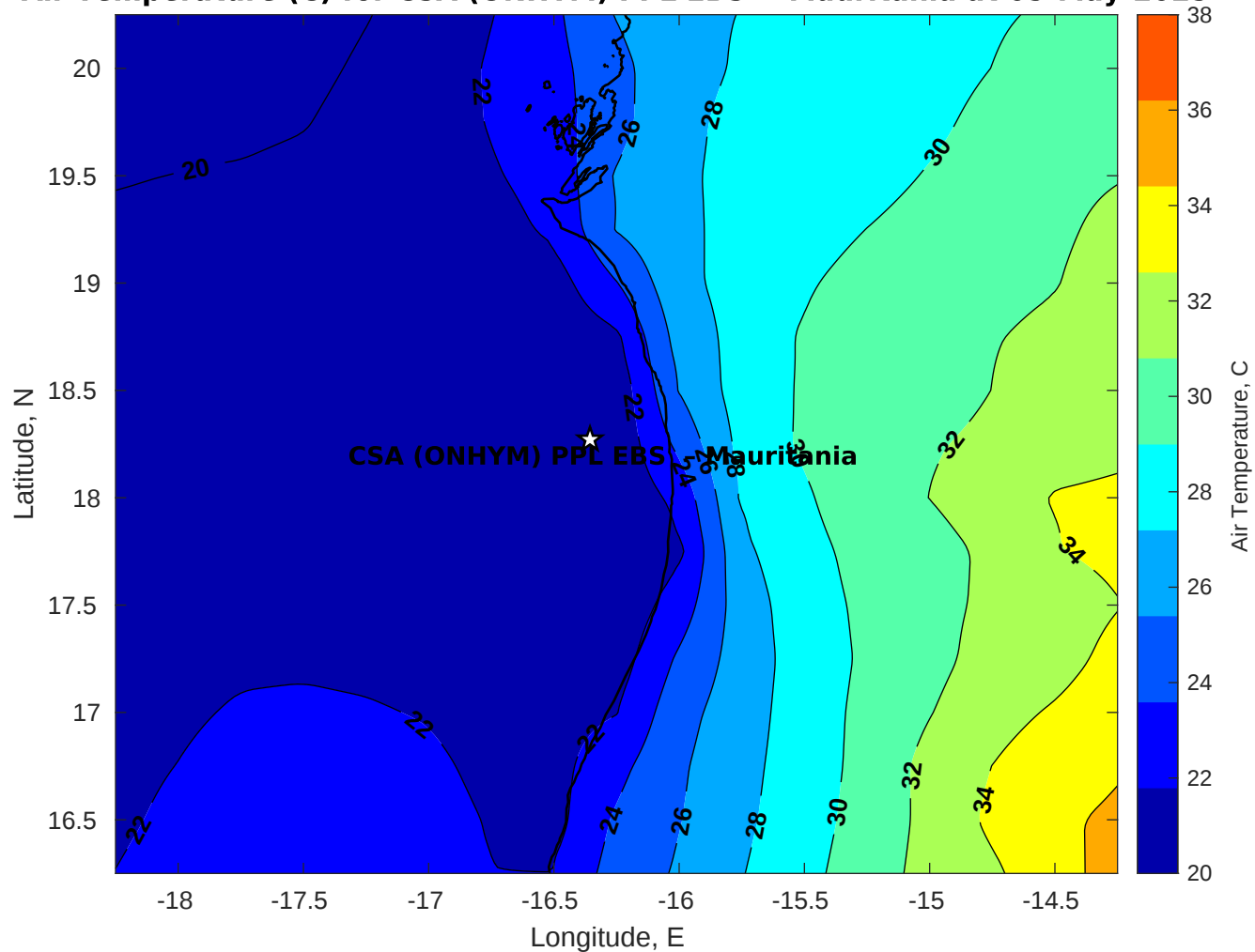
Air Temperature (C) for CSA (ONHYM) PPL EBS - Mauritania at 05-May-2025
